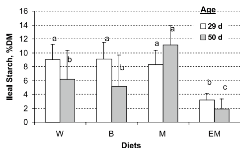
Figure 1. Ileal starch concentration according to age and to dietary starch source. Means and standard error, for eight replicates per diet and per age. Within age, means among diets having a superscript in common are not different at the level P = 0.05 .
