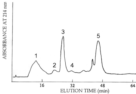
Figure 1. HPLC separation of polypeptides contained in the water-soluble fraction of S. cerevisiae culture. Different peaks are identified with numbers.
