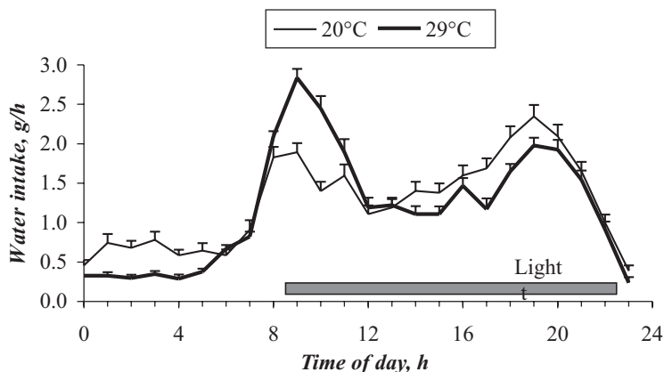
Figure 2. Effect of ambient temperature and time on the kinetics of water consumption (mean + standard error); each point is the mean of 15 sows at 20 °C and 18 sows at 29 °C.
