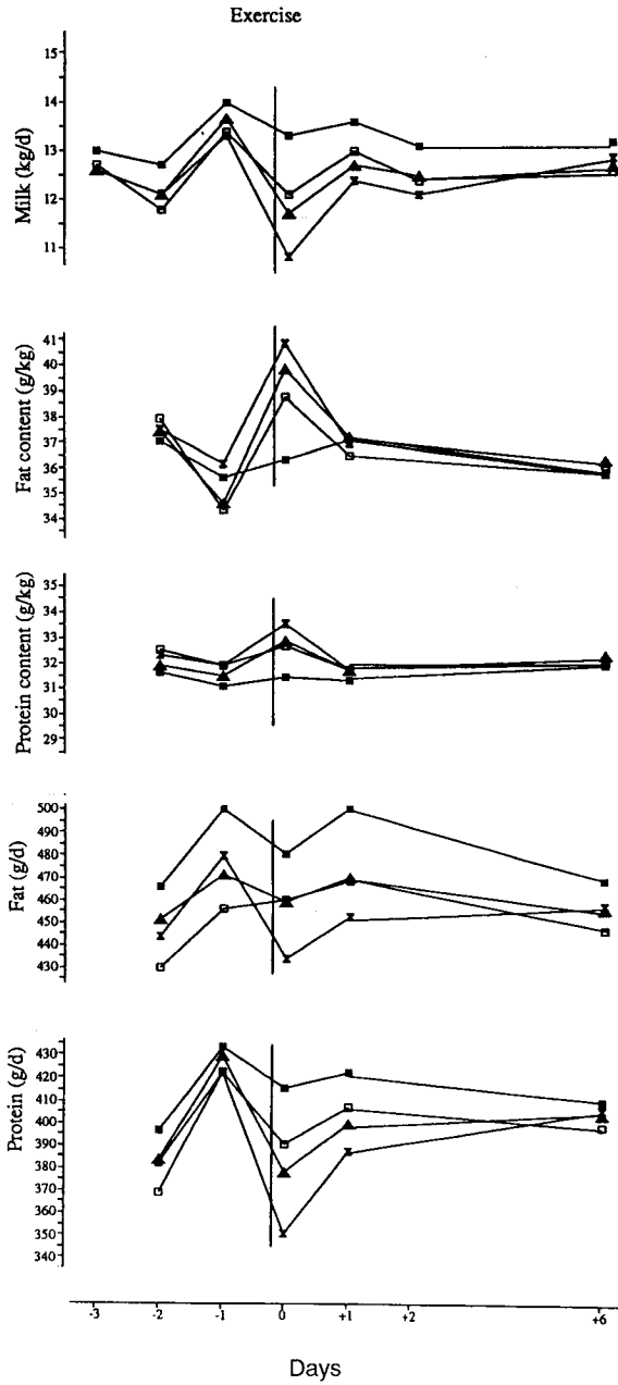
Fig 1. Mean daily milk production and milk composition in dairy cattle before and following walking. 0 (—■—), 6.4 (—□—), 9.6 (—▲—) and 12.8 (—▼—) km.
