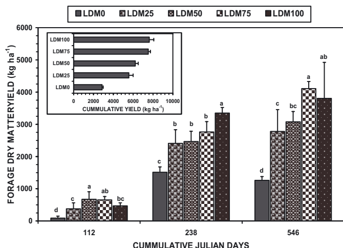
Figure 10. Forage yield of bahiagrass (Julian days 112 to 546) as affected by varying levels of dredged materials application. Forage yield from plots with or without lake-dredged materials are significantly different ( P \leq 0.05 ) at Julian days 112, 238, and 546 when superscripts located at top of bars are different (Source: Sigua, 2008).
