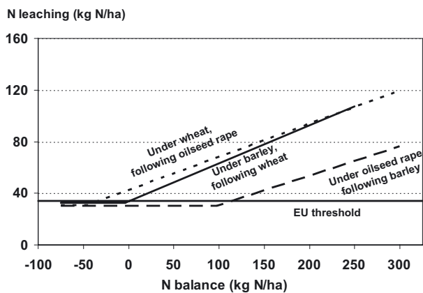
Figure 1. Relationship between N balance (kg N/ha) and annual N leaching (kg N/ha) during the subsequent leaching period in different preceding crop – crop combinations (1991/92–1999/2000). The EU drinking water threshold (50 ppm nitrate) is given for 300 mm percolation (Sieling and Kage, 2006).
