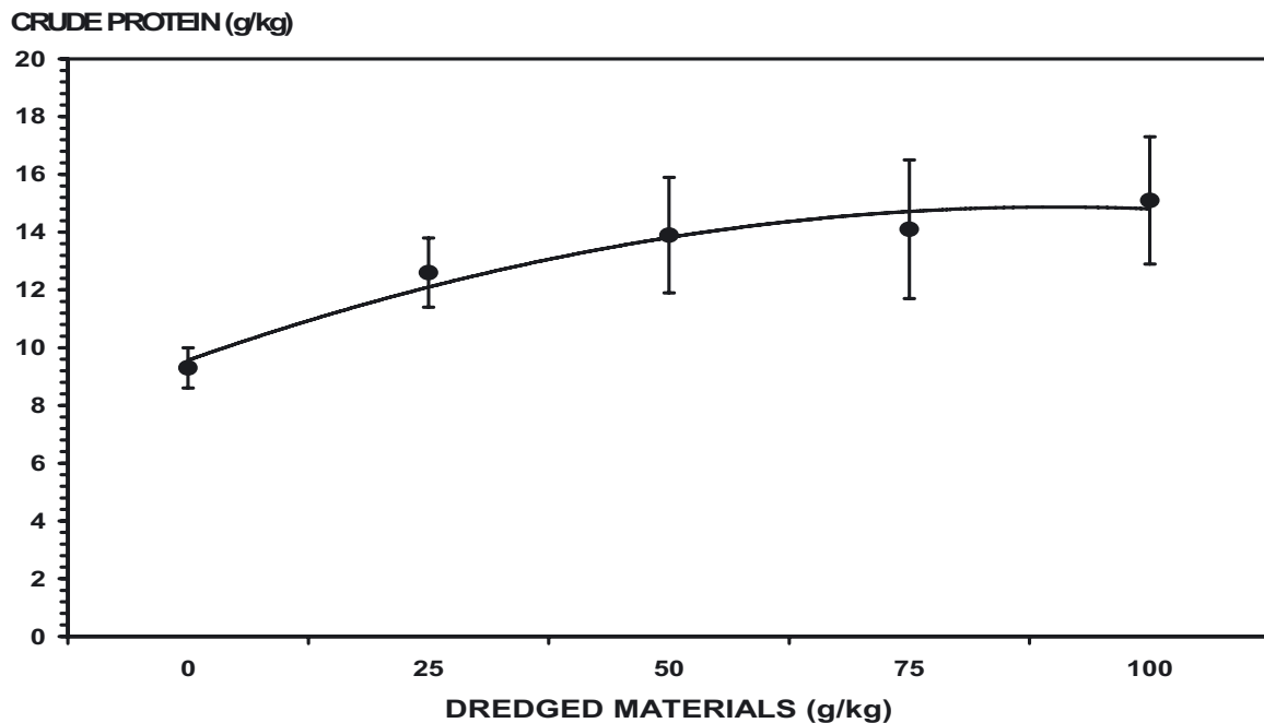
Figure 7. Relationships of crude protein content of bahiagrass with increasing rates of lake-dredged materials application. y = -0.4071DM^2 + 3.7529DM + 6.22 , R^2 = 0.96 ; P \leq 0.0001 .
