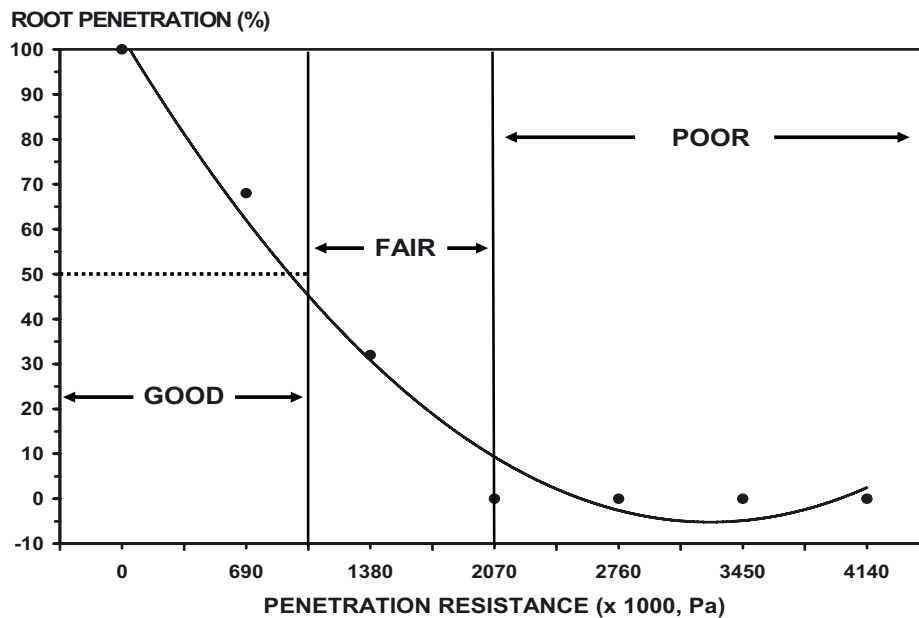
Figure 5. Relationship of root penetration and penetration resistance in soils using penetrometer (Source: Murdock L., Gray T., Higgins F., Wells K. (1995) Soil compaction in Kentucky, Cooperative Extension Service, Univ. Kentucky, Lexington, AGR-161). RP (\%) = 153.1 + 4.8x^2 - 55.2x , R^2 = 0.98 .
