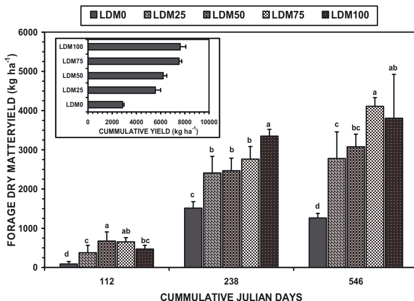
Figure 6. Forage yield of bahiagrass (Julian days 112 to 546) as affected by varying levels of dredged materials application. Forage yield from plots with or without lake-dredged materials are significantly different ( P \leq 0.05 ) at Julian days 112, 238, and 546 when superscripts located at top of bars are different. (Source: Sigua et al., 2004b).
