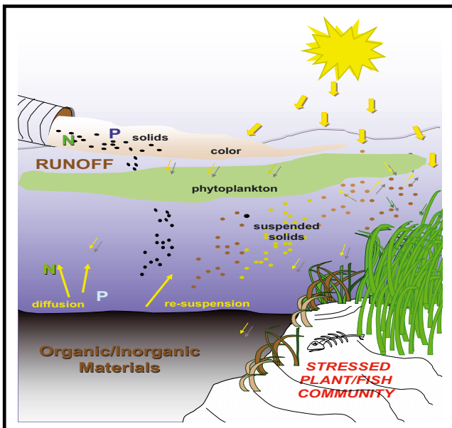
Figure 1. Typical sedimentation process, building up shallow spot called shoals.
