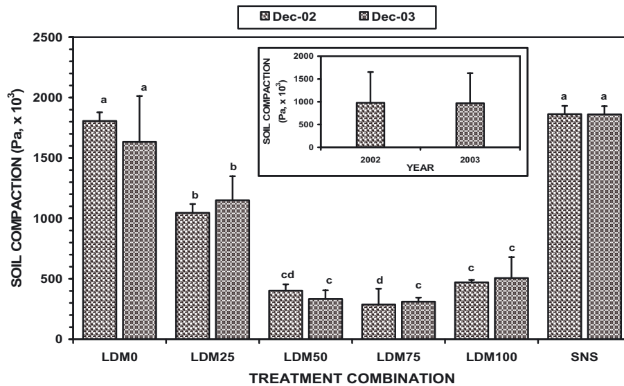
Figure 4. Degree of soil compaction for soils with varying levels of lake-dredged materials. Soil compactions from plots with or without lake-dredged materials are significantly different ( P \leq 0.05 ) when superscripts located at top of bars are different.
