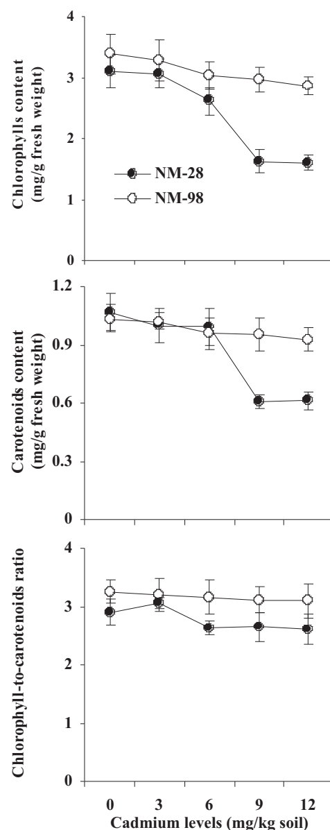
Figure 4. Changes in leaf photosynthetic pigments of mungbean varieties differing in Cd tolerance. These data pertain to the plants treated with increased cadmium levels at the vegetative stage and harvested after 15 days. Pigments were extracted from fresh materials preserved at the time of harvest. Vertical bars are standard deviations of means.
