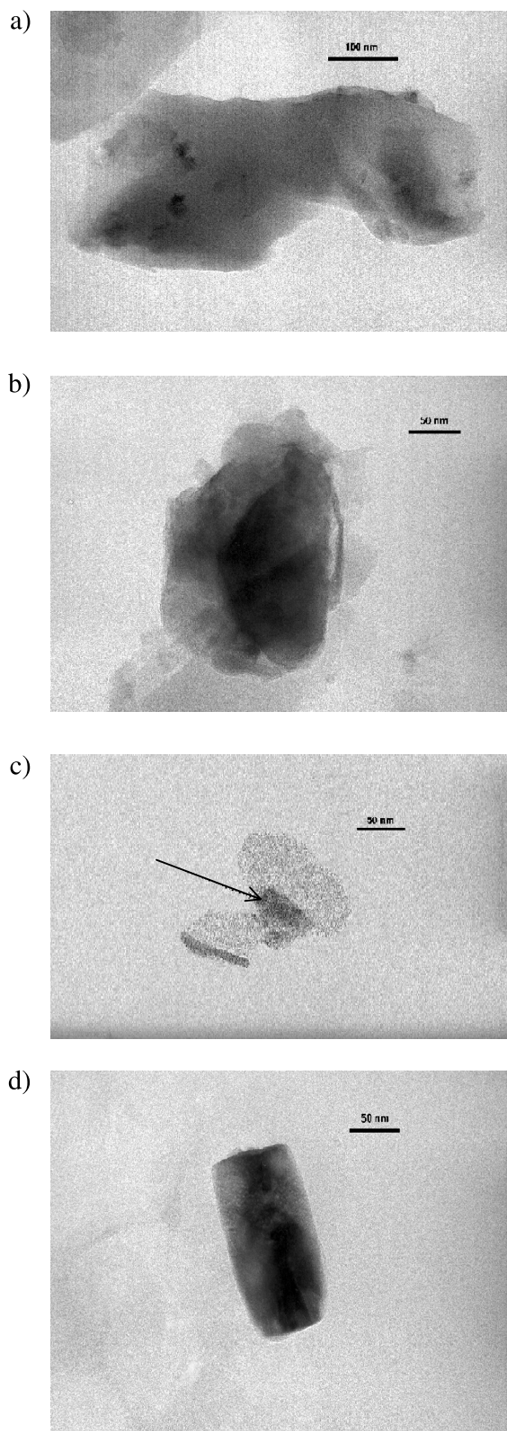
Figure 1. TEM micrographs of soil particles on which silicon dioxide grain (a), silicoaluminate plates (b), aggregates of oxidic iron compounds ( \rightarrow ) on a silicoaluminate plate (c), and titanium dioxide grain (d) are shown.
