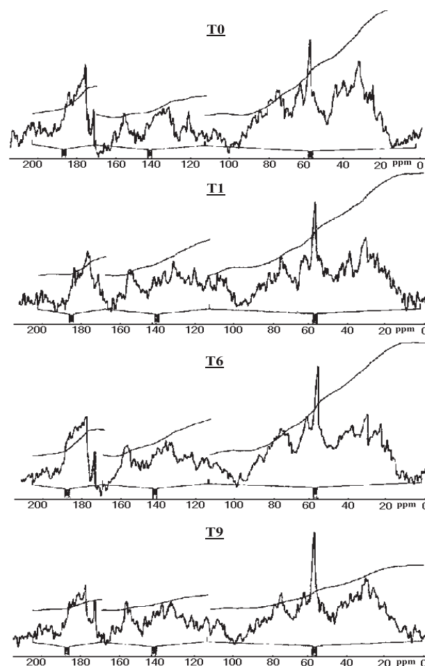
Figure 2. ^{13}\text{C} -NMR spectra of humic acids extracted from the composted sewage sludge at different stages of treatment. Numbers (T0, T1 ... T9) refer to composting time: 0, 1 ... 9 months.
