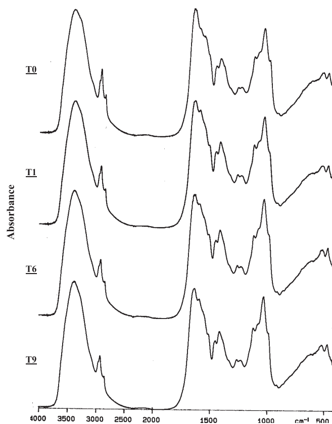
Figure 1. FTIR spectra of humic acids extracted from the composted sewage sludge at different stages of treatment. Numbers (T0, T1 ... T9) refer to composting time: 0, 1 ... 9 months.
