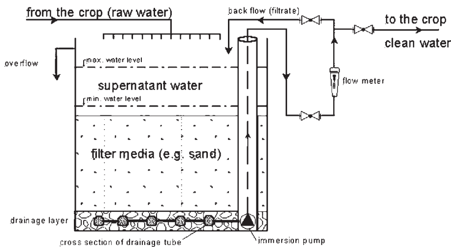
Figure 2. Functional scheme of a slow (sand) filter.
