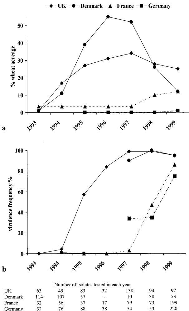
Figure 1. a. Percentage of national wheat acreages growing Yr17 cultivars in Denmark, France, Germany and UK between 1993 and 1999. b. Frequency of virulence for Yr17 in populations of P. striiformis f. sp. tritici in Denmark, France, Germany and UK between 1993 and 1999.
