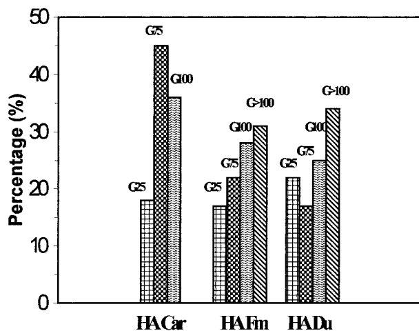
Figure 2. Particle weight distribution of humic acids of composted farmyard manure (HA Fm) and domestic waste (HADu) and of litter (HA Car). Distribution is expressed as percentage of the total weight for each sample of humic acids.
