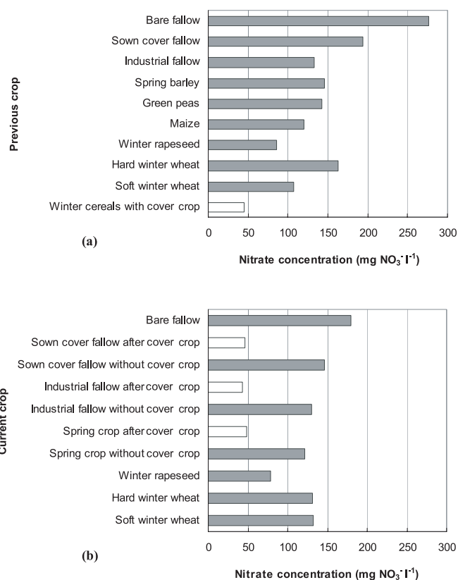
Figure 6. Mean values of nitrate concentration in drainage water according to the (a) previous crop and (b) current crop, over the period 1991–1998.
