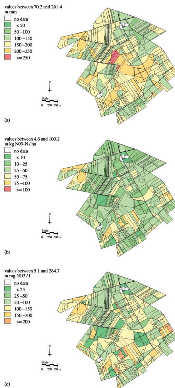
Figure 5. Simulation maps of mean annual values over the period 1991–1998 of: (a) cumulative water drainage, (b) cumulative N leaching, and (c) nitrate concentration in drainage water. Black lines are the borders of the SU.
