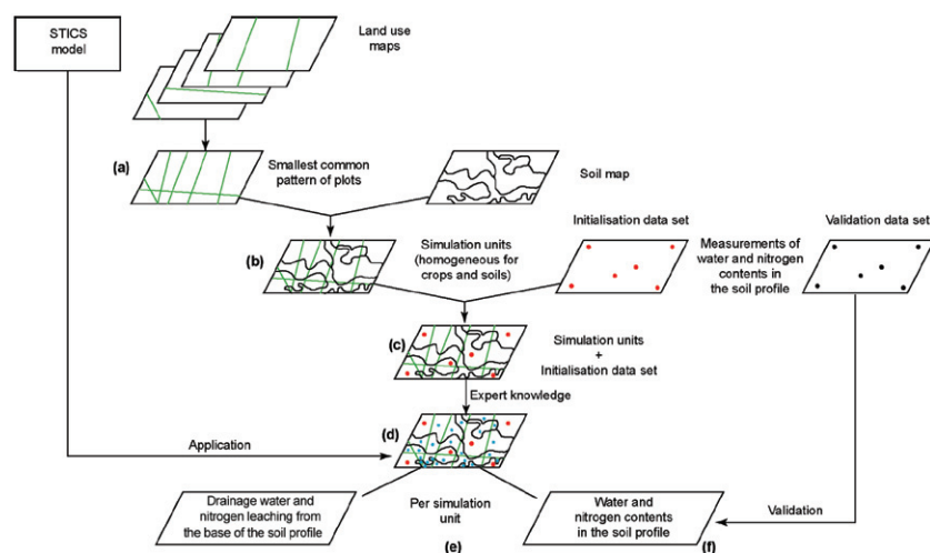
Figure 2. A schematic diagram for upscaling the STICS model.
