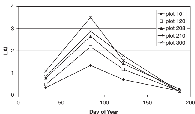
Figure 4. Estimated LAI values derived from SPOT images in 1997 for wheat fields at the Alpillés test site.
