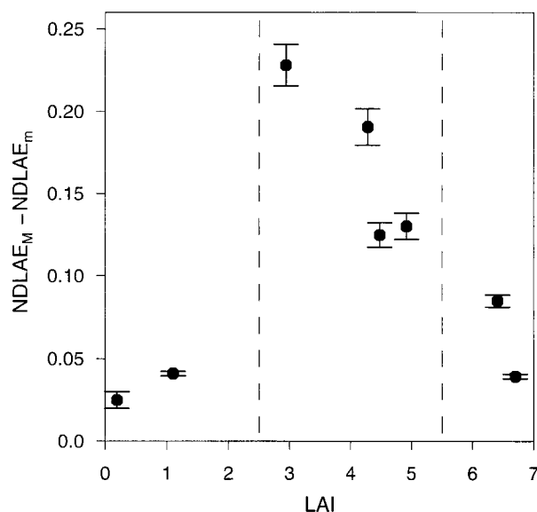
Figure 7. Range of normalized daily light absorption efficiency (NDLAE) calculated with the hypothetical structure generating the highest NDLAE ( \text{NDLAE}_M ) while generating the lowest NDLAE ( \text{NDLAE}_m ). The eight points correspond to the eight canopies described in table I . For each plot, mean and standard deviation are calculated with the six daily incident radiation characteristics shown in table II .
