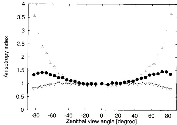
Figure 12. Directional variations of downward fluxes (scattering order > 1 ) at three elevations expressed as the LAI above the considered level: (▲) LAI = 0.5, (●) LAI = 2 and (▽) LAI = 3.7.
