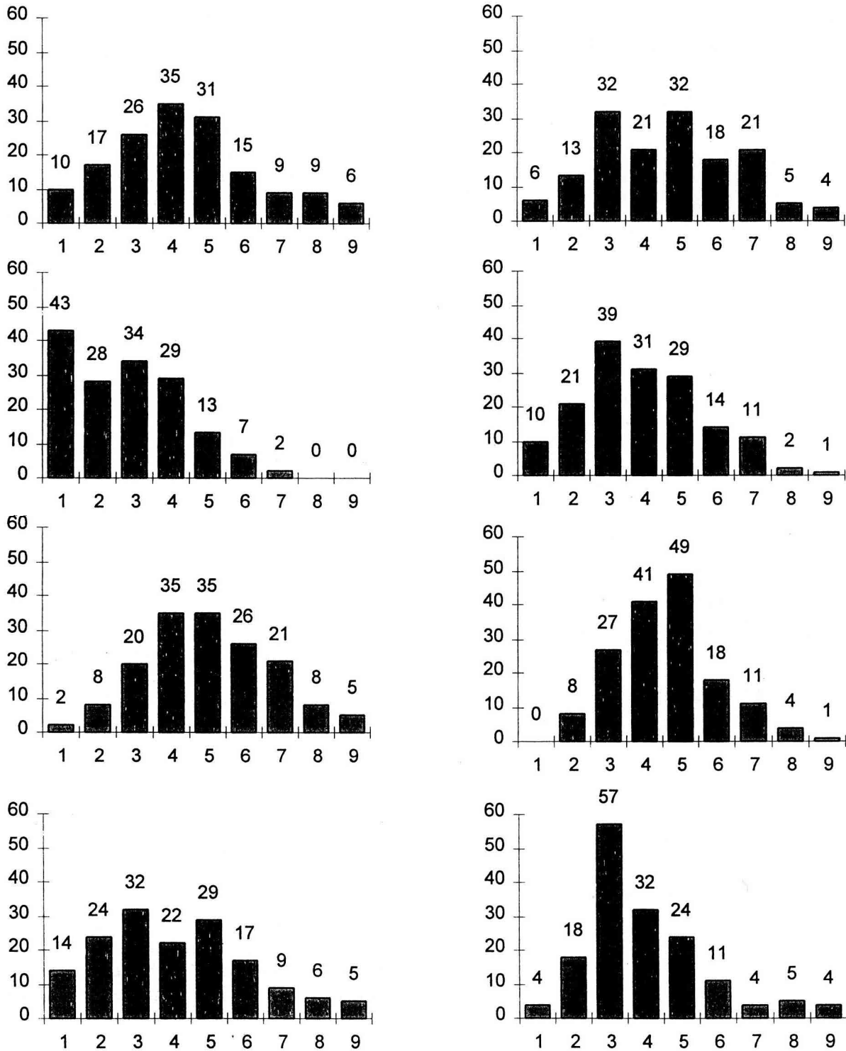
Figure 2. Distribution of eight different experts notation with regard to the pairs of inbred lines at flowering time. The notation estimates the relatedness between the inbred lines. It ranges from 1 (very related) to 9 (very different) and it is averaged over two repetitions.
