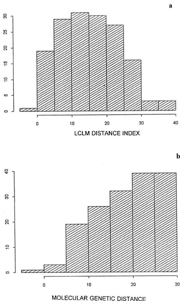
Figure 1. Distribution of the LCLM distance (a) and the molecular genetic distance (b) among the 160 pairs of maize inbred lines of the study.
