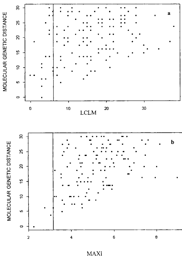
Figure 4. Relationship between the molecular genetic distance and the morphological distances (a) LCLM, and (b) MAXI. (a) The vertical line represents the LCLM = 6 threshold. (b) The vertical line represents the arbitrary threshold of MAXI = 3.15.
