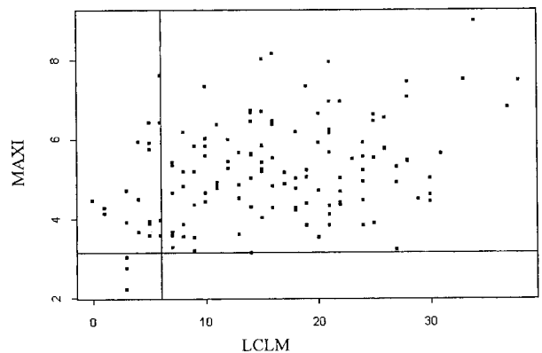
Figure 3. Relationship between the LCLM distance index and the expert's distance (MAXI). The vertical line represents the LCLM = 6 threshold. The horizontal line represents the arbitrary threshold of MAXI = 3.15.
