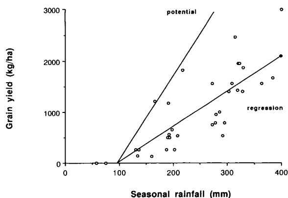
Fig 5. Grain yields versus seasonal rainfall. The slope of the upper line gives the average transpiration efficiency in this climate. The lower line is the regression relation (equation [4]).
