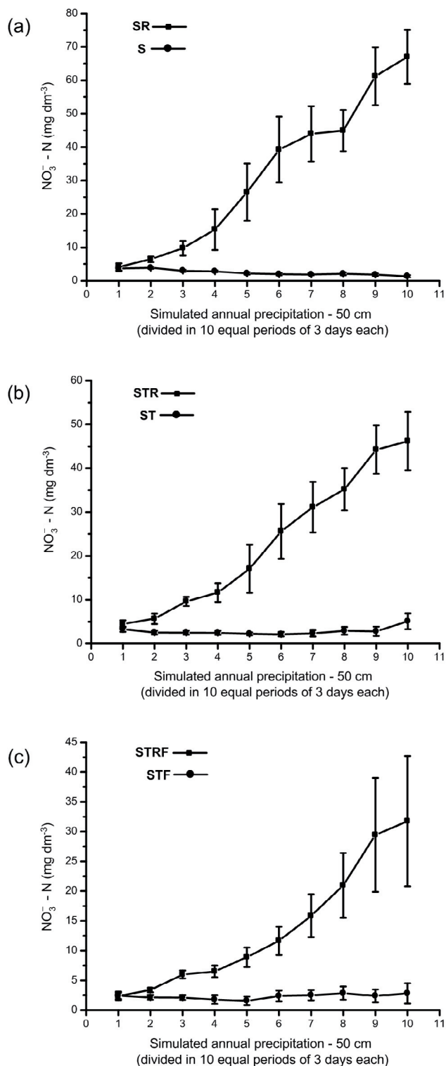
Figure 2. Concentration of \text{NO}_3^- -N in leachates from treated with the retardant pots and their controls, without a tree: SR and S (a), with a tree: STR and ST (b) and with a tree which was subjected to fire STRF and STF samples (c), during a simulated annual precipitation 50 cm. The mean and \pm S.E. of the measurements resulting from replicate experiments (seven for treated samples and four for their controls) are shown at each point of the elution curve.
