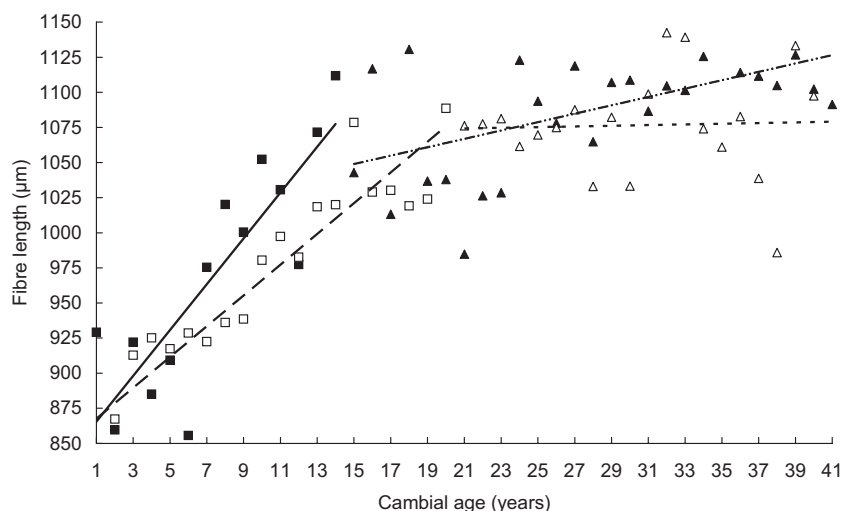
Figure 9. Fibre length increased significantly with cambial age. In trees from the M'voun plantation, the breakpoint between JW and AW was 14.5 y (black squares, solid line: 0–14.5 y: y = 16.30x + 849.4 , R^2 = 0.71 , P < 0.001 . Black triangles, solid + dotted line: 15–41 y: y = 2.45x + 1069.1 , R^2 = 0.001 , P = \text{ns} ). In trees from the Bokoué plantation, the breakpoint between JW and AW was 20 y (white squares, hatched line: 0–20 y: y = 10.96x + 856.7 , R^2 = 0.87 , P < 0.001 . White triangles, dotted line: 21–41 y: y = 2.96x + 1003.6 , R^2 = 0.31 , P = 0.003 ).
