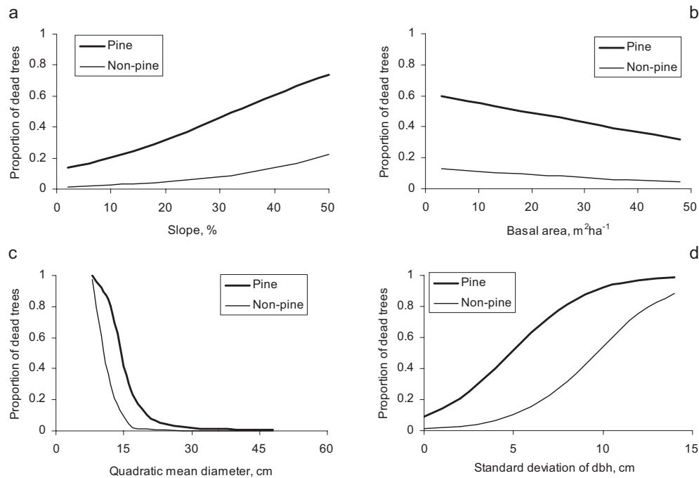
Figure 2. Effect of slope (a), stand basal area (b), quadratic mean diameter (c), and standard deviation of diameter (d) on the proportion of dead trees according to Equation (2). Variables other than the one on the \times axis are equal to their mean value in the modelling data (Tab. II).
