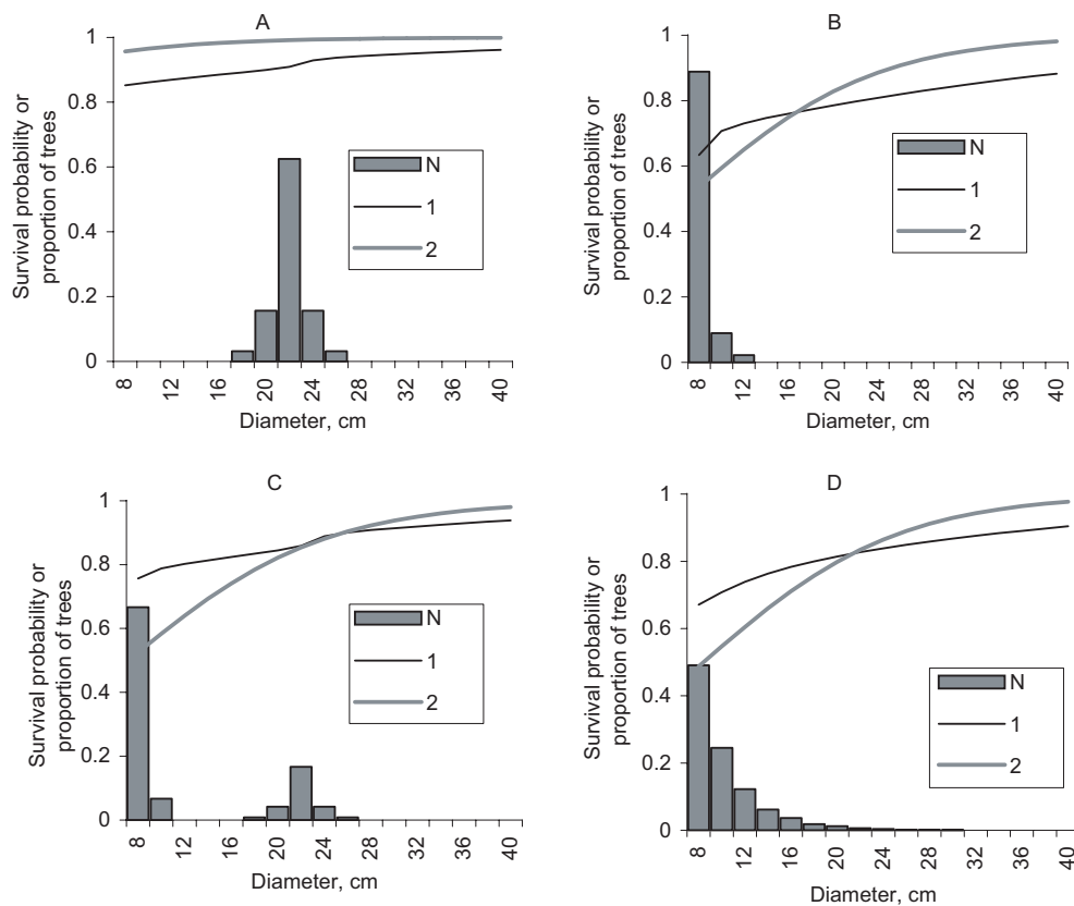
Figure 7. Survival probability and relative number of trees for different diameter classes in an even-aged mature (A), young even-aged (B), two-storied (C), and uneven-aged (D) pine stand that has been swept by fire. The survival probability has been calculated in two ways: (1) with a model in which the degree of damage is not a predictor (Eq. (3)), and (2) using a model (Eq. (4)) in which the predicted degree of damage (Eq. (2)) is used as a predictor. The slope of the terrain was 10 degrees.
