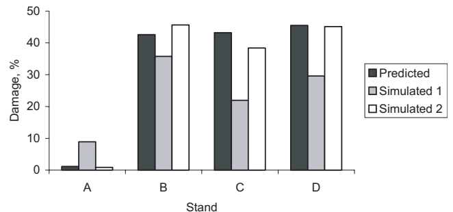
Figure 8. Predicted (Eq. (2)) and simulated damage for the same stands (A,B,C,D) as in Figure 6. The simulated damage is calculated using the survival probabilities of individual trees. Numbers 1 and 2 refer to the calculation method: method 1 uses survival function in which stand level damage is not a predictor (Eq. (3)) while method 2 uses a model (Eq. (4)) where the predicted stand level damage degree is a predictor.
