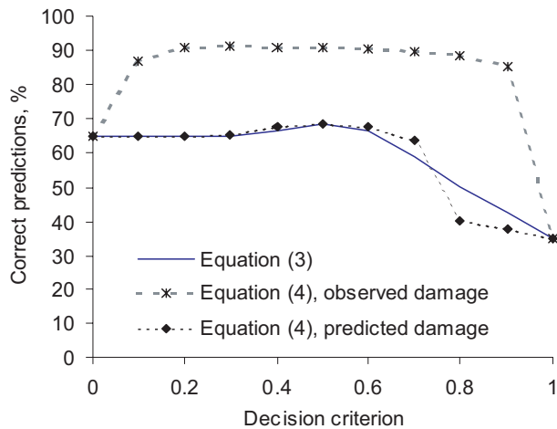
Figure 6. Percentage of correct predictions as a function of predicted survival probability that classifies trees as survivors (decision criterion).
