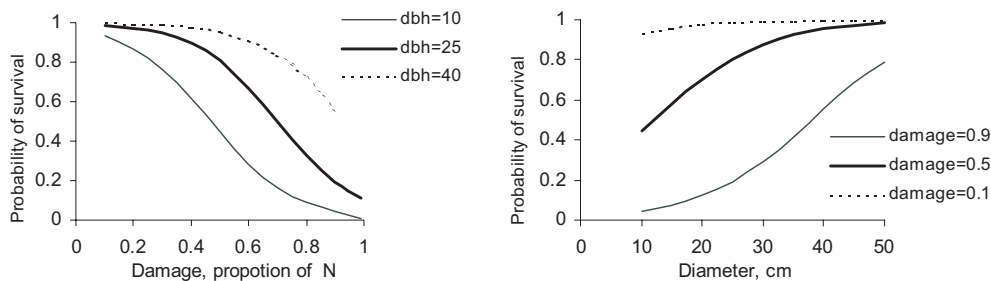
Figure 4. Effect of the degree of fire damage (proportion of dead trees, P_{dead} ) and tree diameter (dbh) on the survival probability of a tree, according to Equation (4).
