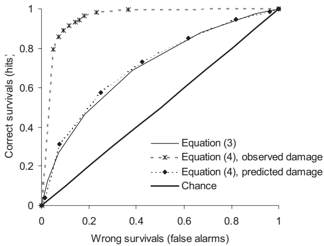
Figure 5. Receiver operating characteristic curves for Equation (3) and for Equation (4) when used with predicted or observed stand level damage. A high area between the x axis and the curve implies high accuracy.
