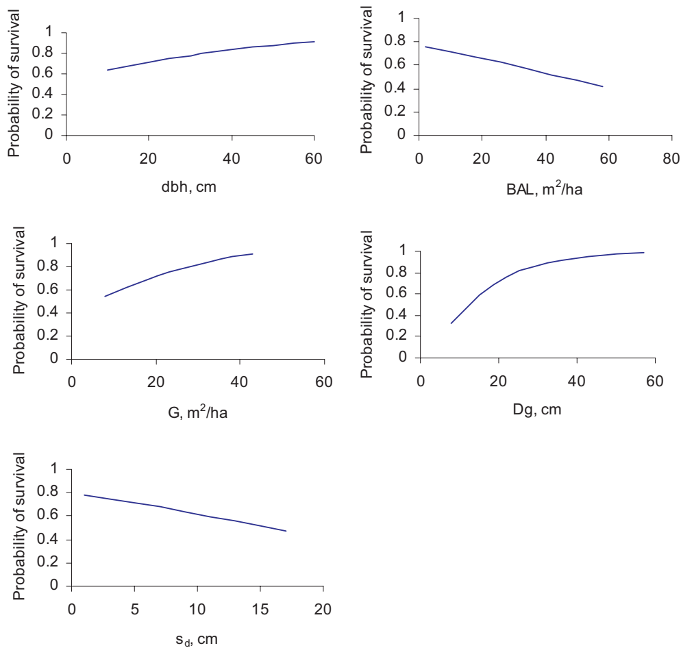
Figure 3. Effect of tree diameter (dbh), basal area of larger trees (BAL), total basal area (G), basal-area-weighted mean diameter (Dg) and standard deviation of dbh ( s_d ) on the survival probability of a tree, according to Equation (3) for species other than P. pinea and Q. suber .
