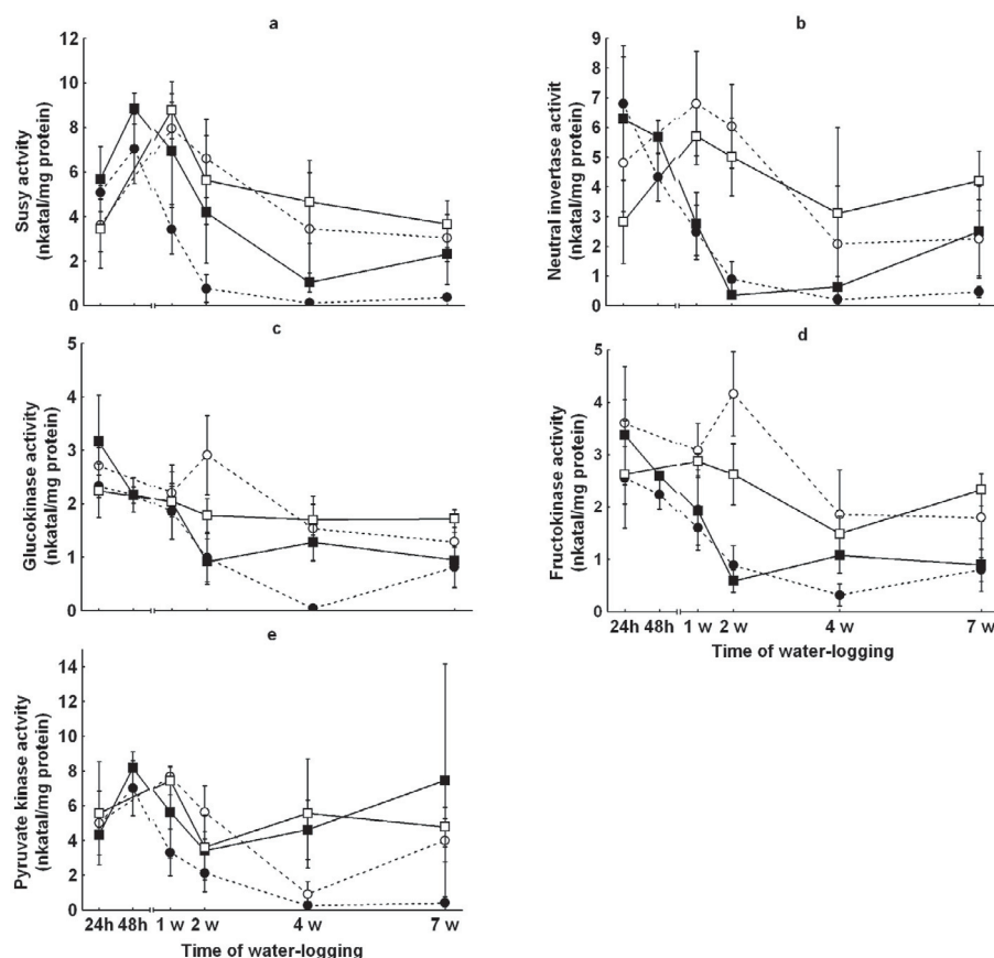
Figure 5. Specific enzymatic activities of the carbon catabolism in fine roots (nkatal mg -1 protein, means and SEM, n = 5 except for control at 24 h: n = 3 ). (a) Susy activity. (b) INV-7.5 activity. (c) GK activity. (d) FK activity. (e) PK activity. w: weeks; same symbols as in Figure 1.
