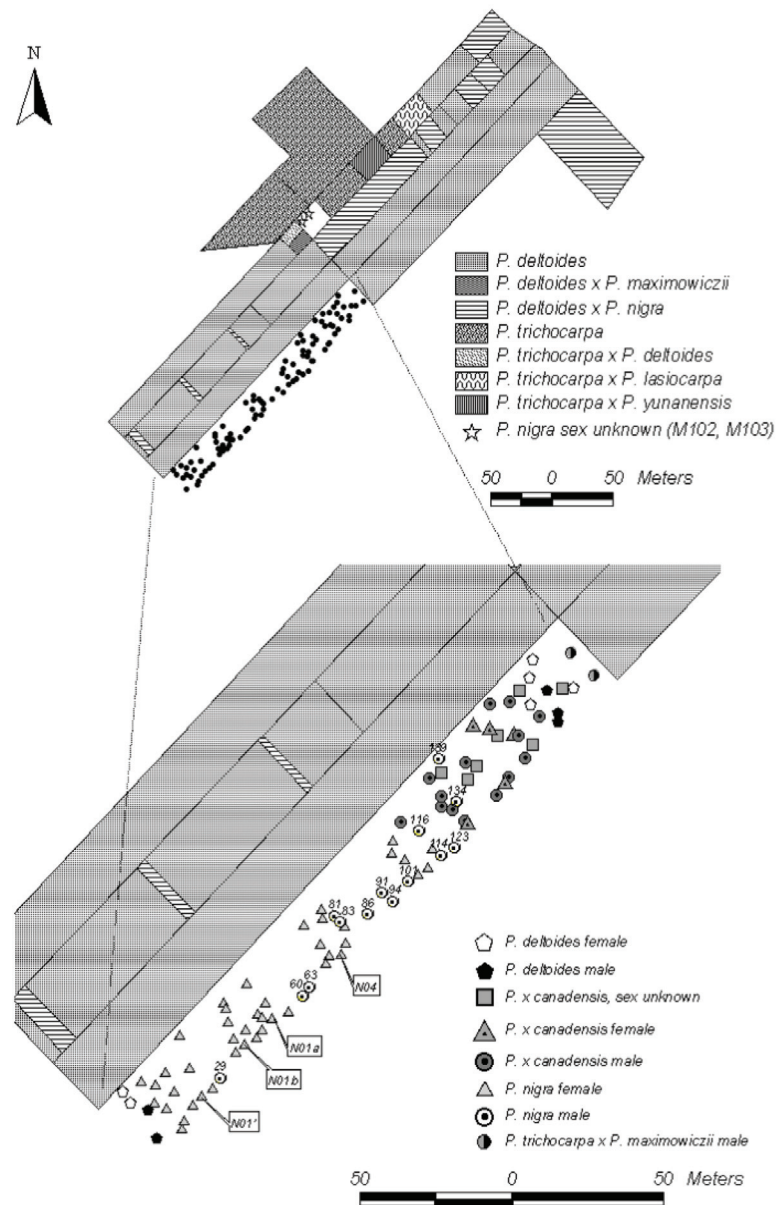
Figure 1. Location and species composition of the study site in the poplar plantation ‘Marcq’. The location of the four P. nigra mother trees N01a, N01b, N01’ and N04 sampled are labelled, the male black poplar trees are indicated by a number.
