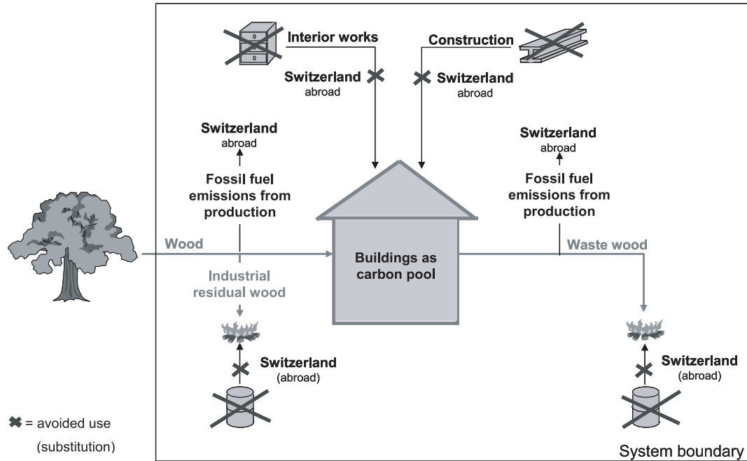
Figure 1. System boundaries of the building stock and its respective GHG effects.
