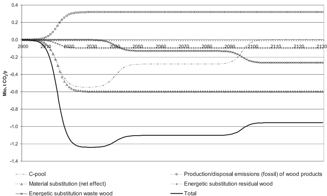
Figure 7. GHG emissions dynamics of an increased use of wood (2000–2130).
