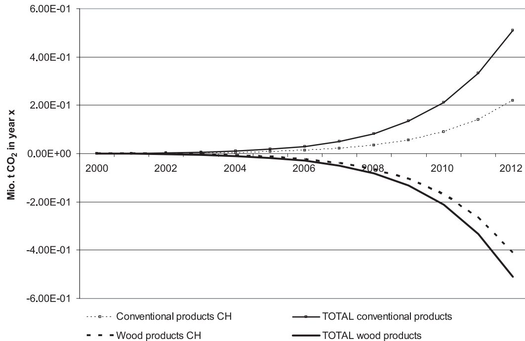
Figure 10. Scenario ‘conventional’ products instead of wood products 2000–2012 (cumulated flows).
