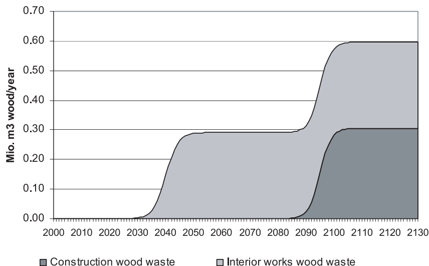
Figure 3. Increased waste wood flows in the years 2000 to 2130.
