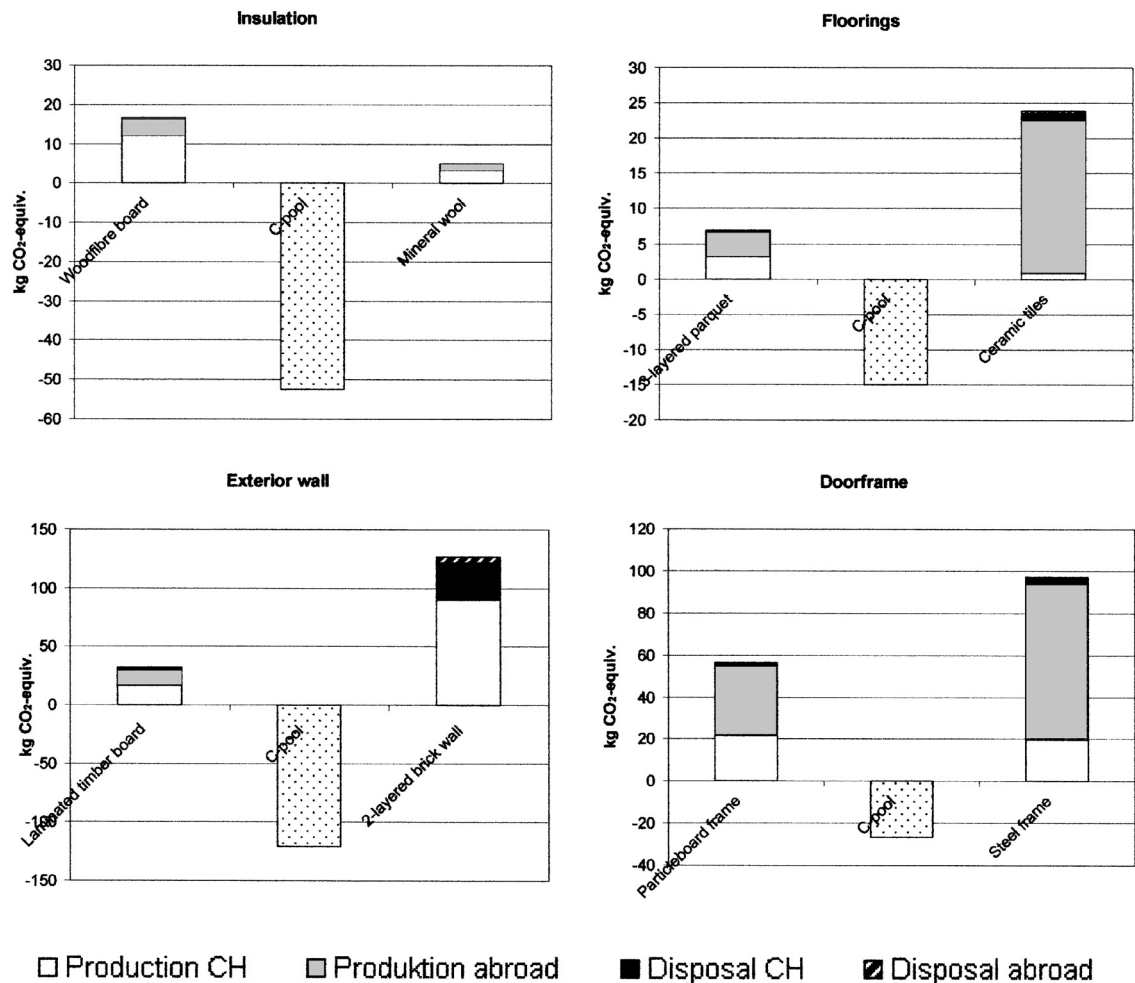
Figure 5. Selected product-specific potential carbon pool capacities, production emissions and substitution effects, in Switzerland (CH) and abroad.
