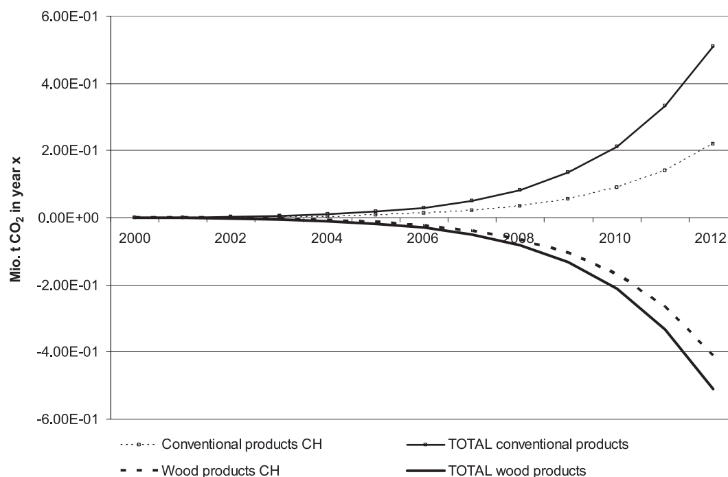
Figure 10. Scenario ‘conventional’ products instead of wood products 2000–2012 (cumulated flows).
