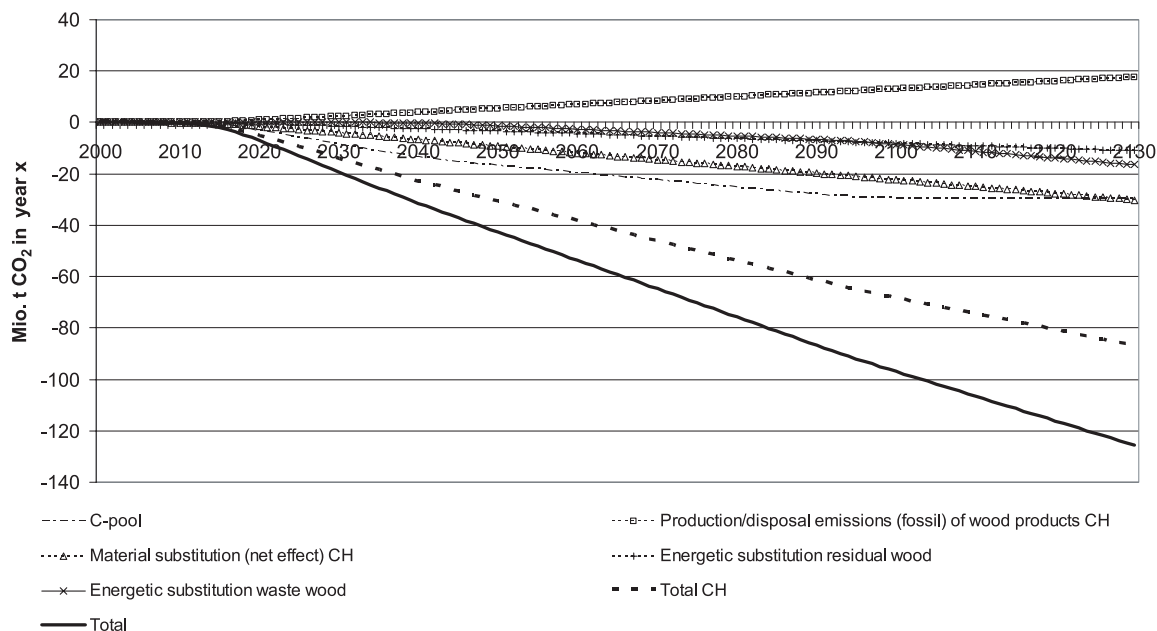
Figure 9. Cumulated GHG effects of an increased use of wood in Switzerland (2000–2130).
