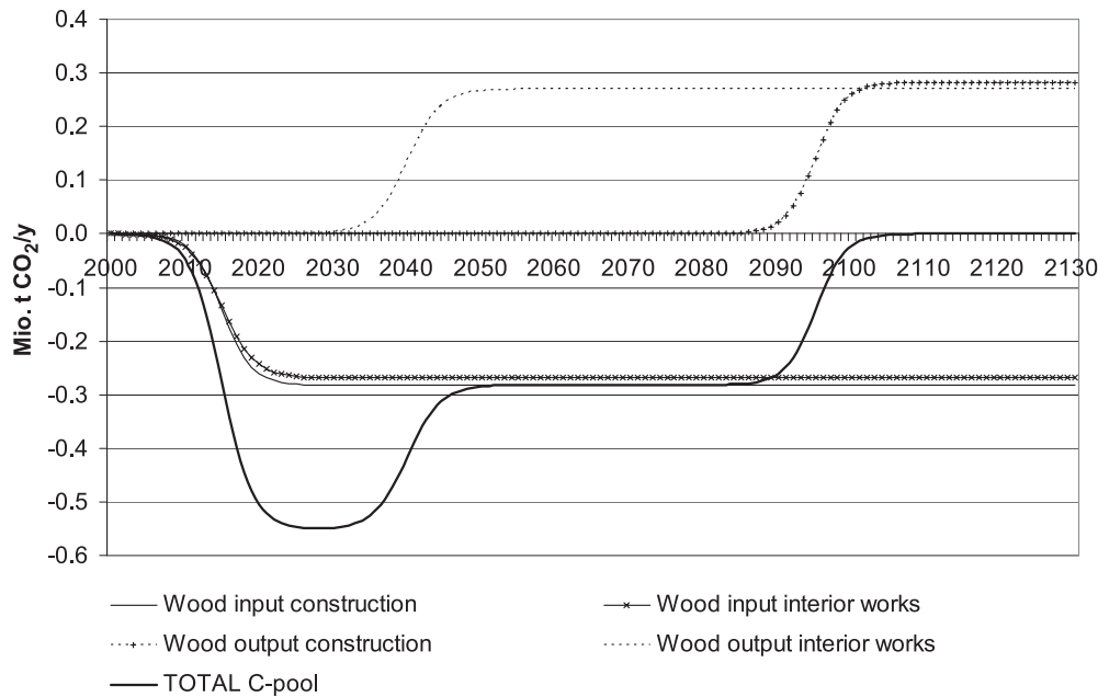
Figure 4. Dynamics of the building stock as carbon pool 2000 to 2130 (annual flows).
