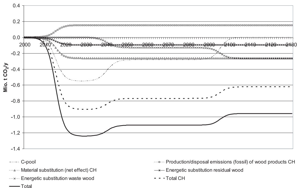
Figure 8. Annual GHG flows in Switzerland due to an increased use of wood (2000–2130).
