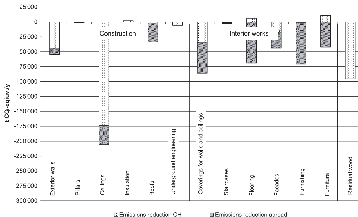
Figure 6. Substitution effects of different wood products due to an increased use of wood, in Switzerland (CH) and abroad (+ 0.81 Mio. m 3 of wood).
