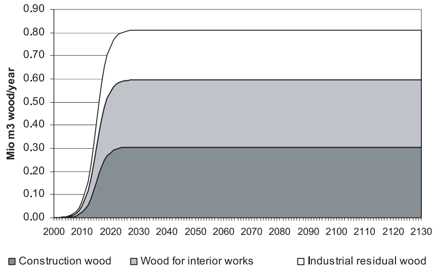
Figure 2. Increased use of wood flows in the years 2000 to 2130.
