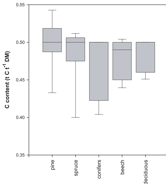
Figure 3. Box plots (see Fig. 1 for detailed description) of carbon content values for different tree species (groups); only species for which more than 5 CC values were available are presented.
