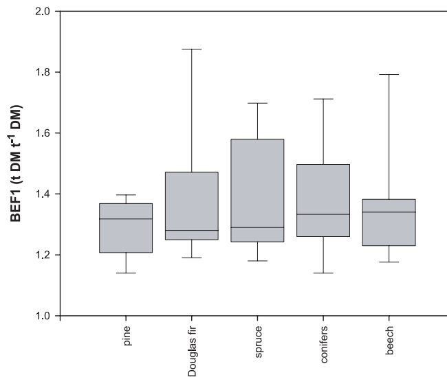
Figure 2. Box plots (see Fig. 1 for detailed description) of BEF1 values for different tree species (groups); only species for which more than 5 BEF1 values were available are presented.
