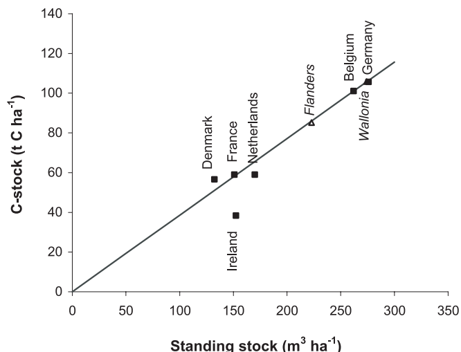
Figure 4. Relation between standing stock ( \text{m}^3 \text{ha}^{-1} ) and carbon stock ( \text{t C ha}^{-1} ) for Belgium and neighbouring countries; the solid line gives the C-stock when the overall Belgian BEF s.l. is used.
