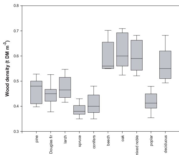
Figure 1. Box plots of wood density values for different tree species (groups); the horizontal line within each box represents the median value for each species (group). Each box contains 50% of the observed values within the limits of the first and the third quartile. Error bars indicate 10 and 90% quartiles.
