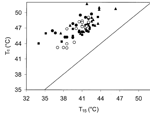
Figure 2. Relationship between T_{15} and T_c recorded on needles of four different conifers. The linear correlation was statistically significant ( n = 20 , r = 0.72 , p < 0.05 ). Current year needles of P. nigra (open disks), P. halepensis (squares), C. sempervirens (plain disks) and C. atlantica (triangles). The 1:1 line was drawn for clarity.
