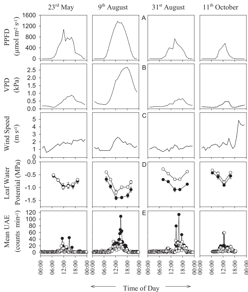
Figure 2. Diurnal variation of physiological and meteorological variables during four days over the experimental period, in 1995: (A) photosynthetically active radiation (PAR), (B) air vapour pressure deficit (VPD), (C) wind speed, (D) leaf water potential ( \Psi_L ), and (E) ultrasonic acoustic emissions in branches (UAE). The first three columns represent days during the progression of the drought, the final column is after the end of the drought period. Closed symbols: water-stressed trees, open symbols: controls. Error bars indicate \pm 1 standard error.
