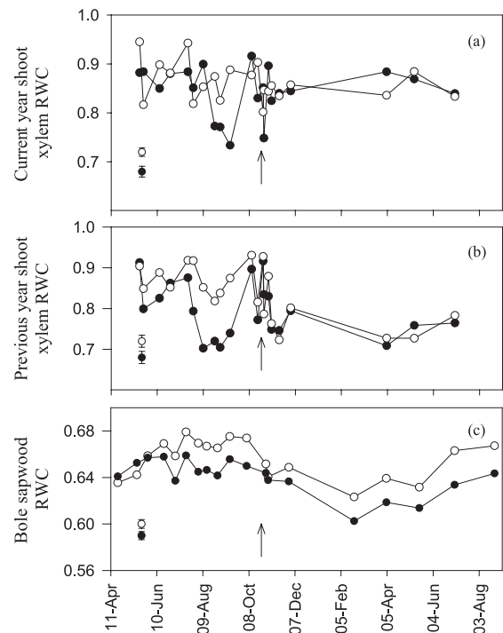
Figure 5. Seasonal variation in the relative water content ( R_w ): (a) current year shoots, (b) previous year shoots, and (c) bole sapwood (to 5 cm depth), during the drought year (1995). Closed symbols: water-stressed trees, open symbols: controls. Points are mean values. The arrows indicate the rewatering date when the water-stress plot was returned to field capacity. Error bars indicate \pm 1 standard error, n = 4 .
