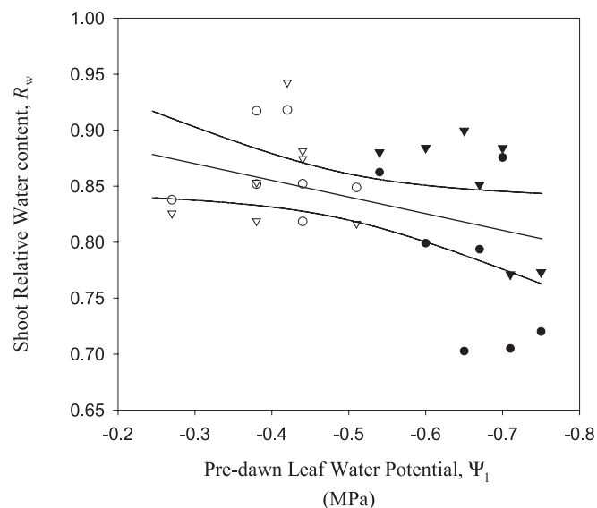
Figure 6. Relative water content ( R_w ) in the twig xylem as a function of pre-dawn leaf water potential ( \Psi_{LPD} ) ( R_w = 0.94 + 0.19 \Psi_{LPD} ). 95% confidence intervals are reported ( r^2 = 0.21 , p < 0.05 ). Data presented is up to and inclusive of 31st August. Closed symbols: water-stressed trees, open symbols: control trees, circular symbols: current year shoots, triangular symbols: previous year shoots.
