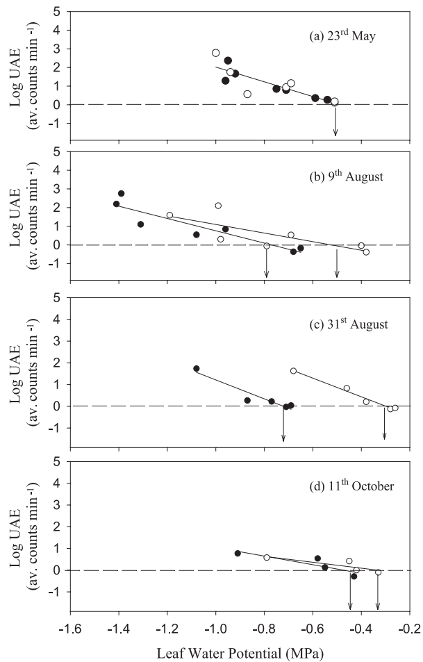
Figure 3. The relationship between mid-day leaf water potential and the log of cavitation rate (data averaged for all plots taken from a 45 min period, corresponding with the time of \Psi_L measurement), indicating vulnerability to cavitation, on four days, during 1995: (a) 23rd May (treatments combined, r^2 = 0.28 ), (b) 9th August (water-stressed, r^2 = 0.34 , watered, r^2 = 0.28 ), (c) 31st August (water-stressed, r^2 = 0.39 , watered, r^2 = 0.40 ), and (d) 11th October (treatments combined, r^2 = 0.31 ). All regressions were significant at \alpha = 0.05 . Closed symbols: water-stressed trees, open symbols: controls. The broken horizontal lines correspond to one cavitation event per minute below which UAE's are deemed indistinguishable from noise.
