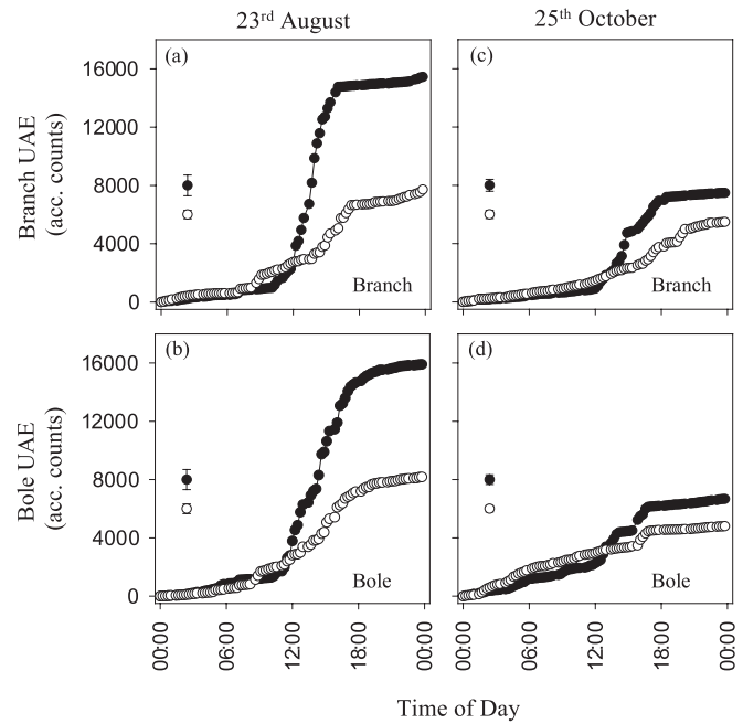
Figure 4. Daily accumulated counts of ultrasonic acoustic emissions in Pinus sylvestris (L.) on two dates over the season: 23rd August in (a) branches, and (b) boles, 25th October in (c) branches, and (d) boles. Closed symbols: water-stressed trees, open symbols: controls. Error bars indicate \pm 1 standard error (grouped data).
