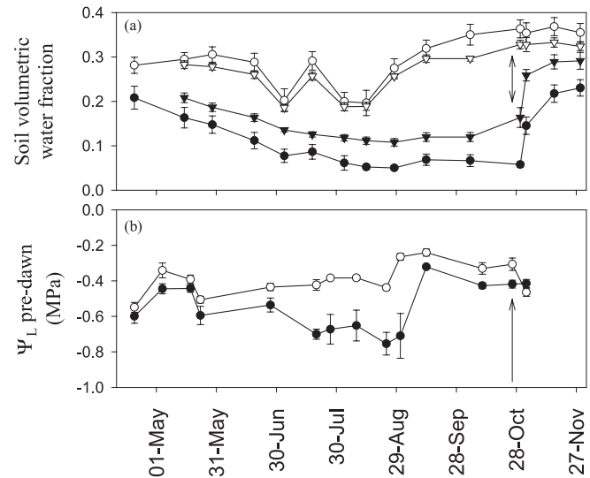
Figure 1. Seasonal variation in (a) soil volumetric water fraction, integrated over the top 20 cm soil depth (circles) and 50 cm soil depth (triangles) ( n = 12 ), and (b) the pre-dawn needle water potential ( \Psi_{L,PD} ) ( n = 4 ). The arrows indicate the rewatering date when the water-stress plot was returned to field capacity. Closed symbols: water-stressed trees, open symbols: controls. Points are means \pm 1 standard error.
