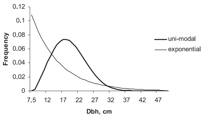
Figure 6. Exponential and uni-modal P. sylvestris diameter distributions of the initial stand when LEV was maximized, for medium site characteristics, 20-year cutting cycle and 2% discounting rate.
