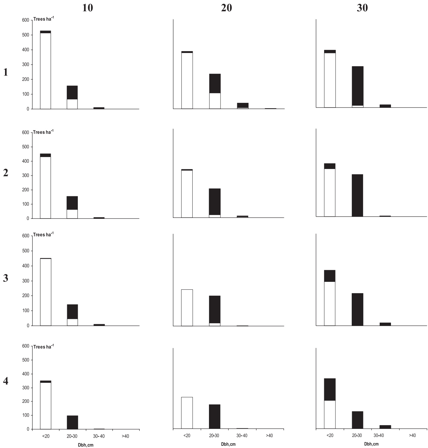
Figure 1. Harvested (black) and residual (white) number of trees per hectare in the four diameter classes used in the study for optimal management with the LEV objective function, different cutting cycles in years (columns) and discounting rates as percentage (rows).
