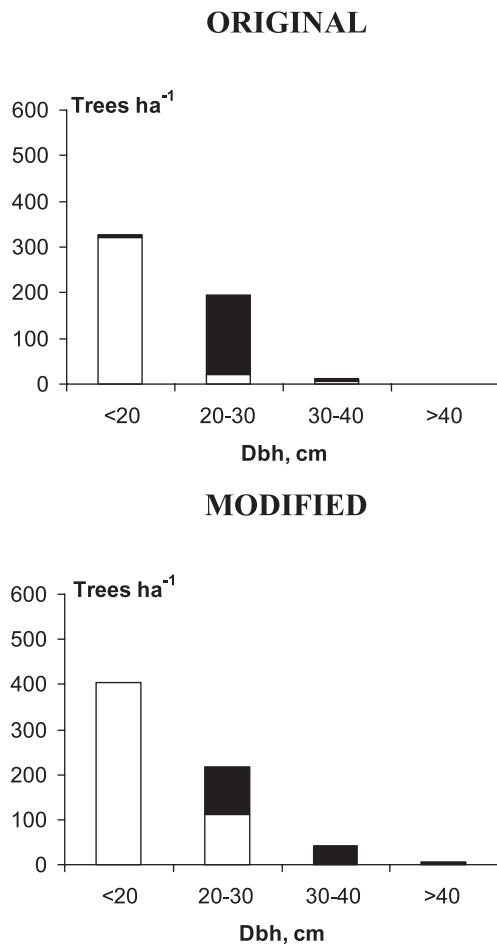
Figure 5. Harvested (black) and residual (white) number of trees per hectare in the four diameter classes used in the present study for optimal management with LEV objective function, the original and modified dbh -price functions and 2% discounting rate percentage.
