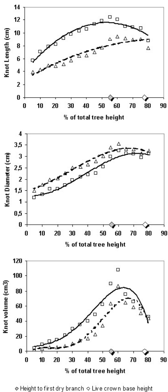
Figure 7. Total (□) and sound (△) knot length, diameter and volume as a function of tree height, as the average for the 20 sampled trees. The corresponding polynomial fitted curves are indicated by (—) for total knot dimensions and by (---) for sound knot dimensions.
