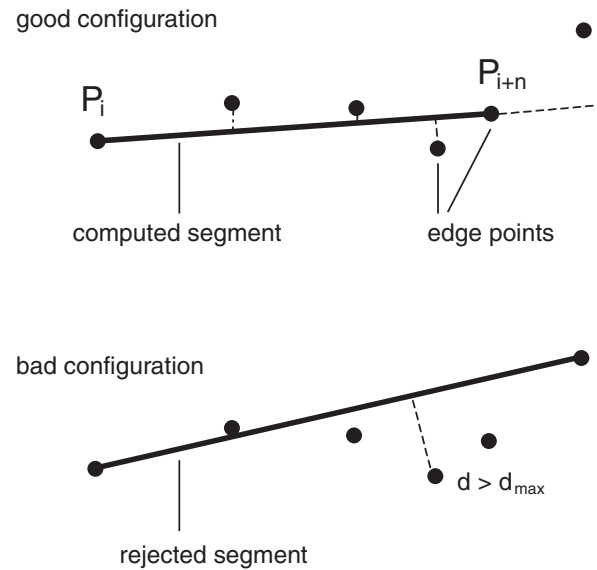
Figure 9. Edge approximation. The segment replaces the edge points if the distance of each removed point to this computed segment is smaller than d_{max} .
