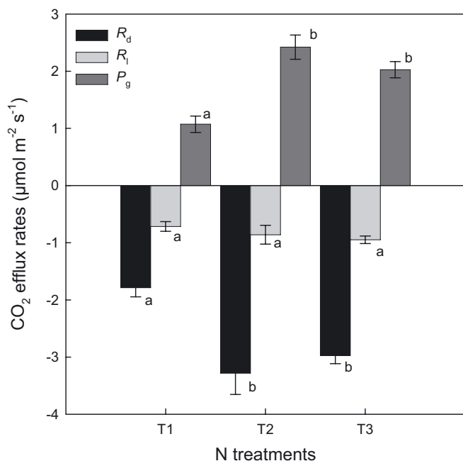
Figure 1. Gas exchange of current-year stems of Fagus sylvatica L. measured as CO 2 efflux in the dark (dark respiration rate, R_d ), CO 2 efflux under saturated light ( R_i ) and calculated rates of gross photosynthesis ( P_g ), for each N treatment (T1, T2, and T3). Data are means \pm 1 SE, with n = 3 . Letters (a, b, and c) indicate significant differences between N treatments, for each parameter ( R_d , R_i and P_g ).
