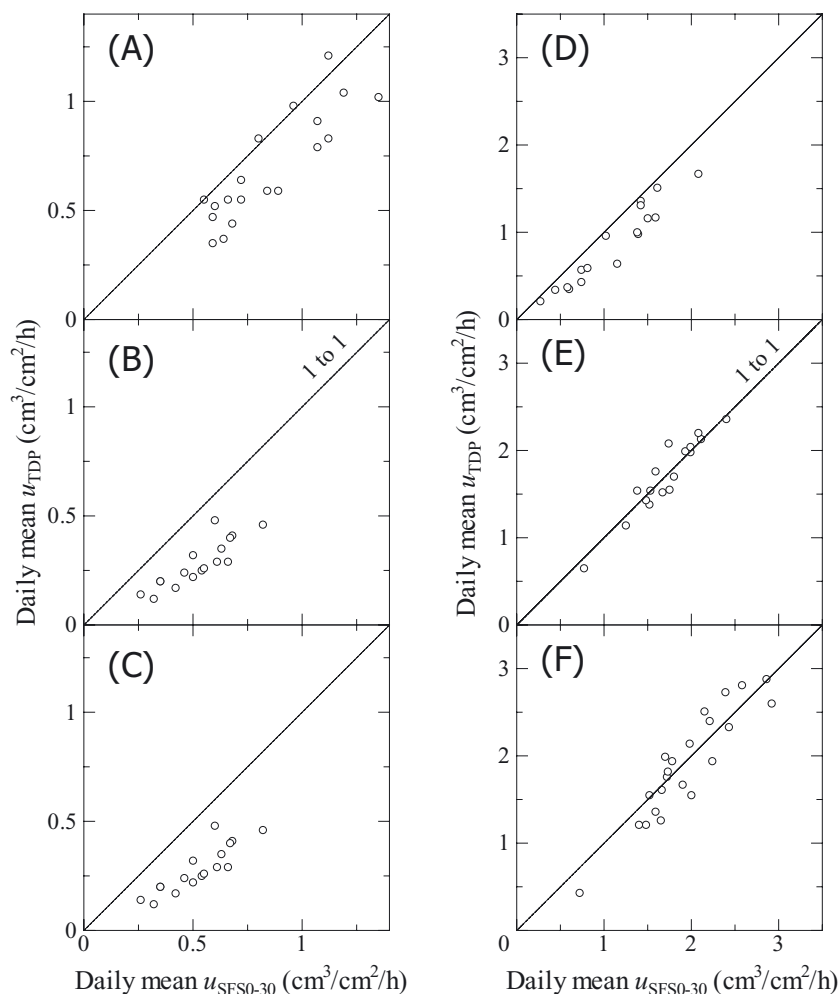
Figure 3. Comparisons of the daily mean values of u between the SFS ( u_{SFS0-30} ) and TDP ( u_{TDP} ) for December 2004 (A), and January (B), February (C), March (D), April (E), and May 2005 (F).
