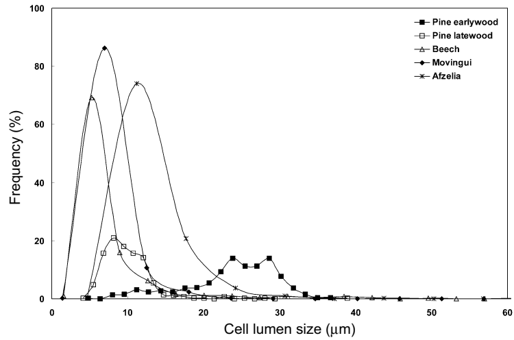
Figure 8. Frequencies of the equivalent diameter of the cell lumen sizes for four wood species.
