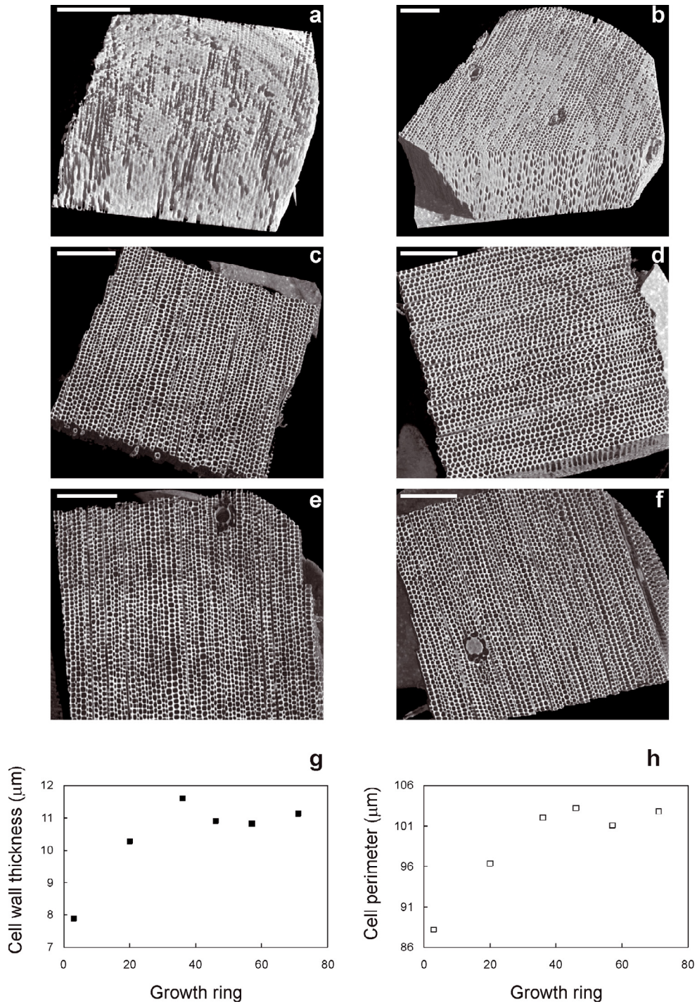
Figure 11. Six reconstructed pine latewood volumes sampled from pith to bark (a-f) and their cell wall thickness (g) and cell perimeter (h) in function of the growth ring they were sampled from. White bar = 400 μm.
