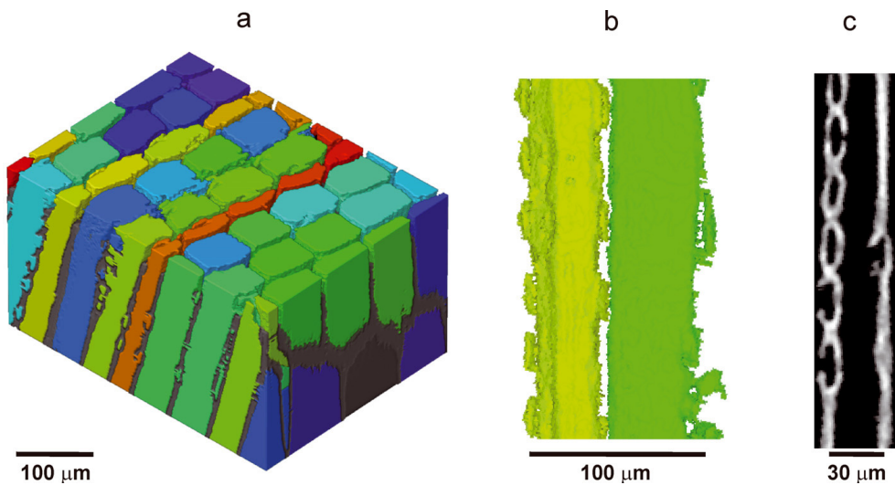
Figure 10. Labelled cell lumens of the noise-free pine earlywood sample with greyish cell wall (a), detailed rendering of pitting between two cells (b) and a 2D slice as an example of the limits of resolution for pit visualization.
