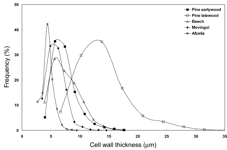
Figure 9. Frequencies of cell wall thicknesses for four wood species.
