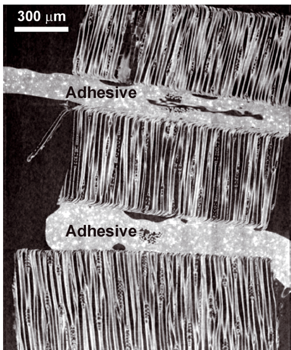
Figure 2. Cross-sectional view through a stack of three pine latewood samples.
