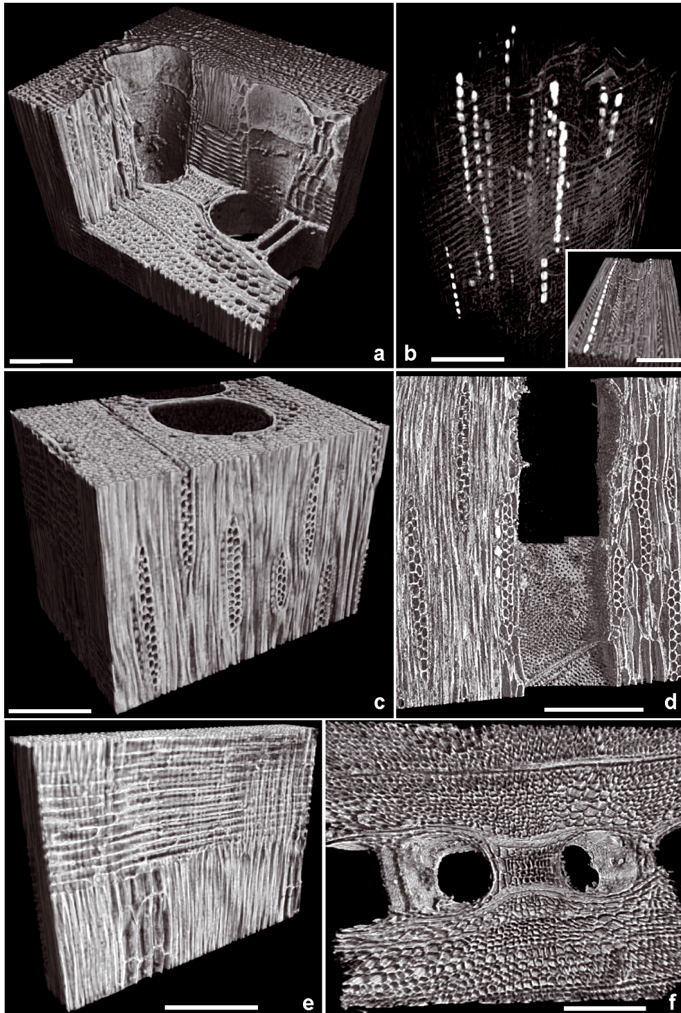
Figure 6. Overview with cut out (a) giving a clear view on the internal anatomy of Afzelia bipindensis Harms; (b) prismatic crystals; (c) rays; (d) simple vessel perforation; (e) view through ray and parenchyma; (f) top view. White bar = 200 \mu\text{m} .
