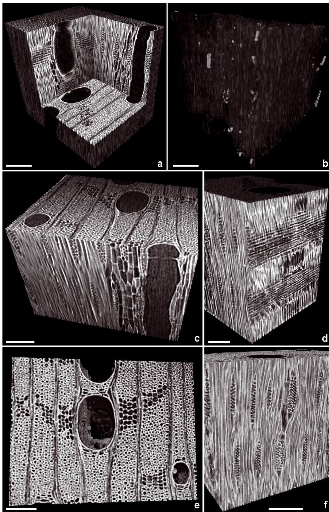
Figure 5. Overview with cut out (a) giving a clear view on the internal anatomy of Distemonanthus benthamianus Baill.; (b) prismatic crystals; (c) parenchyma, rays and slice through vessel; (d) longitudinal slice through rays; (e) top view; (f) tangential view on rays. White bar = 200 μm.
