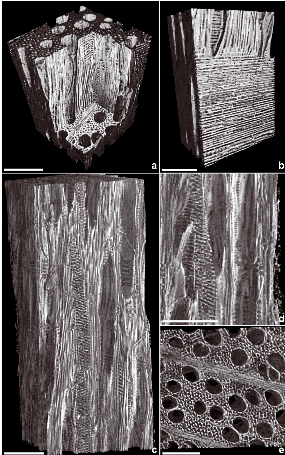
Figure 4. Overview with cut out (a) giving a clear view on the internal anatomy of Fagus sylvatica L.; (b) rays and scalariform vessel-ray pitting; (c) large rays with several vessel cross-sections; (d) perforations of the vessel wall and view on the ray frame; (e) top view. White bar = 200 \mu\text{m} .
