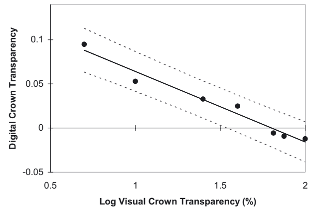
Figure 3. Relationship between Visual and Digital Crown Transparency values obtained with the CROCO computation in 7 poplar trees of contrasted crown transparency. Continuous line indicates the regression fit; dotted line indicates the confidence interval (95%) ( N = 7 , F_{6,1} = 152.0 , P < 0.0001 , R^2 = 0.97 ).
