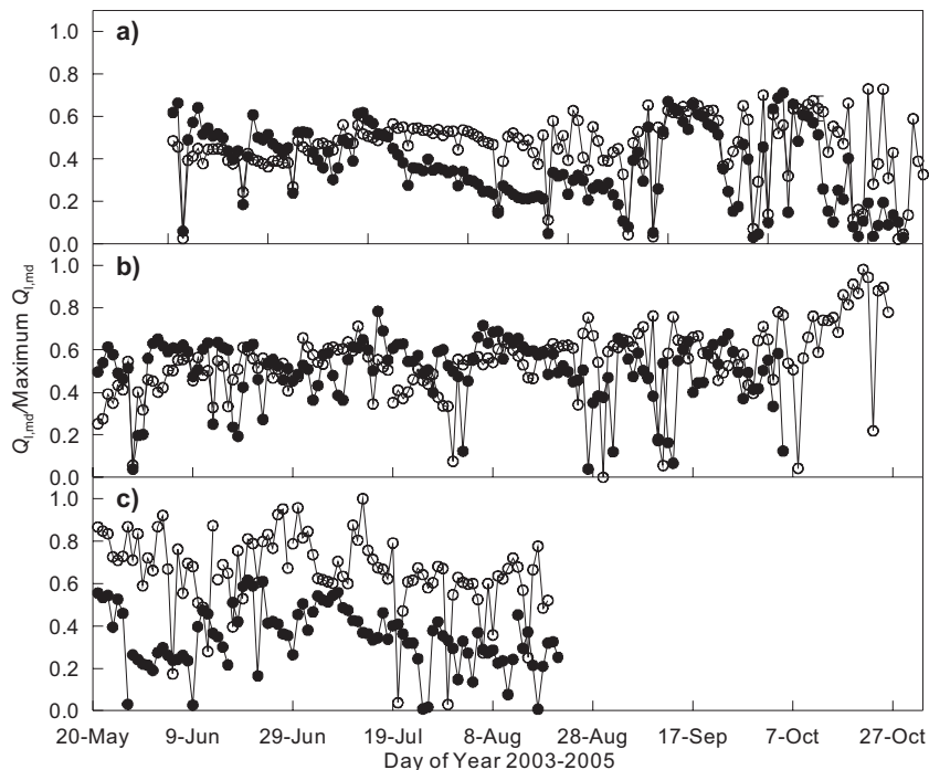
Figure 4. Sap flow per unit leaf area relative to its maximum value for P. sylvestris (closed symbols) and Q. pubescens (open symbols) during (a) 2003, (b) 2004 and (c) 2005.
