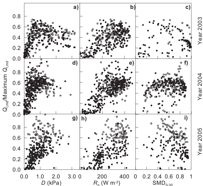
Figure 5. Relationships between relative sap flow and environmental variables for the three years of study for Pinus sylvestris (closed symbols) and Quercus pubescens (open symbols). Panels (a), (d) and (g) show relationships with vapour pressure deficit ( D ); (b), (e) and (h), with net radiation ( R_n ) and (c), (f) and (i) with superficial soil moisture deficit ( SMD_{0-30} ).
