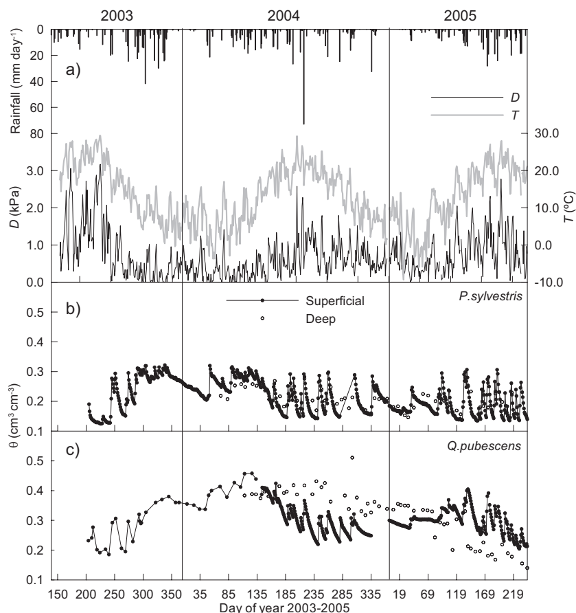
Figure 1. Meteorology and soil moisture during the whole period of study (June 2003–August 2005). (a) Air temperature ( T ) and vapour pressure deficit ( D ) only shown for the pine plot, and rainfall measured in a clearing close to the pine plot. (b, c) Closed dots represent superficial soil moisture ( \theta_{0-30} ), measured continuously or weekly (at the beginning of the monitoring period in the oak plot). Open dots correspond to soil moisture in deeper soil layers measured weekly in both plots ( \theta_{30-50} in the oak plot and \theta_{30-60} in the pine plot).
