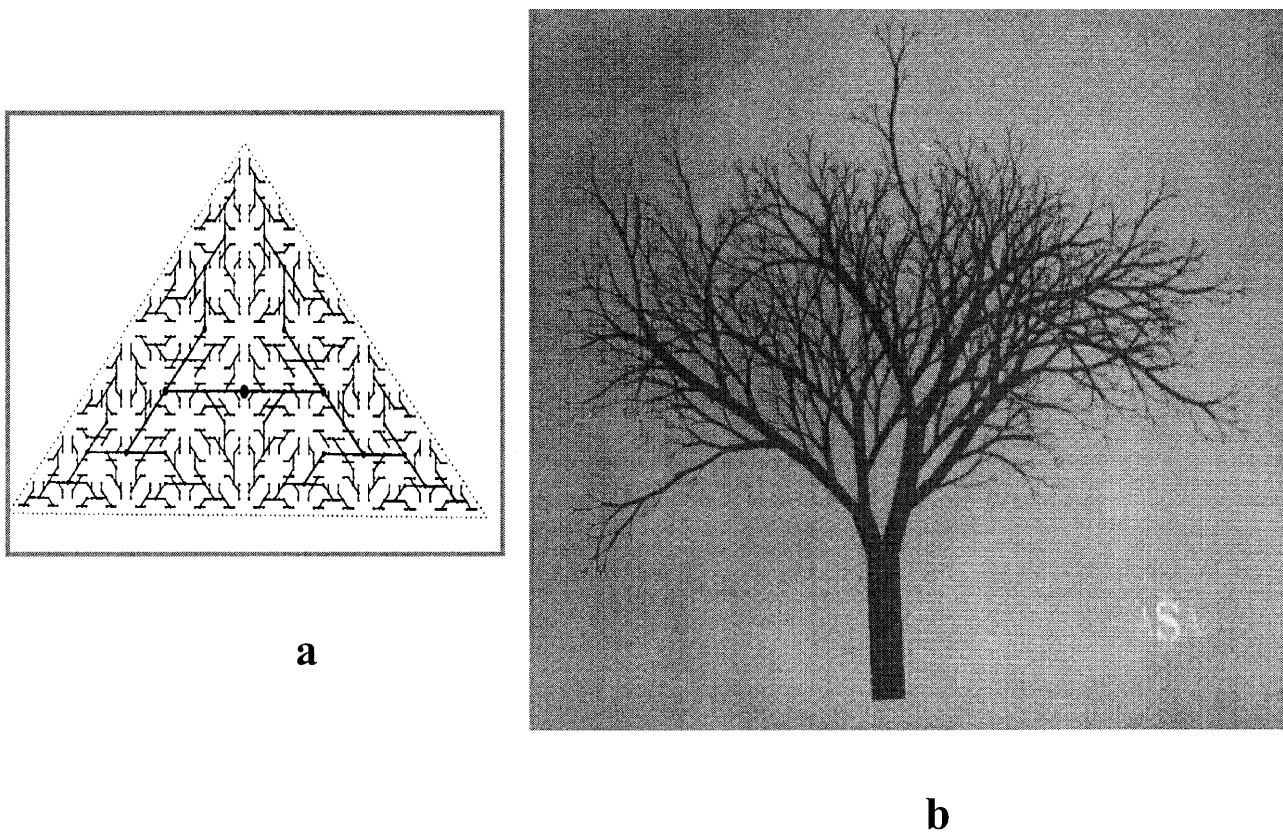
Figure 14. a. Self-similar formal tree resulting from a fractal process. The theoretical output is a fractal object, i.e. it has details at every scale and has an infinite length (from [82]) b. Virtual and realistic tree obtained from a fractal process (e.g. [125], Photo by Viennot).
