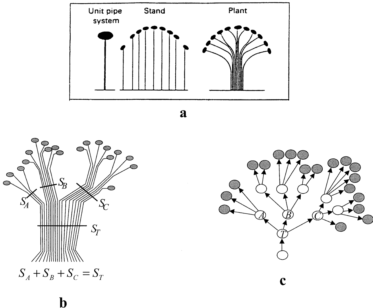
Figure 5. Modular description used with the pipe model theory a . Classical representation of a plant in the pipe model theory (from [107]) b . representation of a branching system with unit pipes: each segment of a tree is represented by a bundle of pipes. A Kirchhoff's current law expresses flux conservation c . Tree graph associated with the model from b . Each bundle of pipe is represented by a vertex and connection between bundles is represented by an edge.
