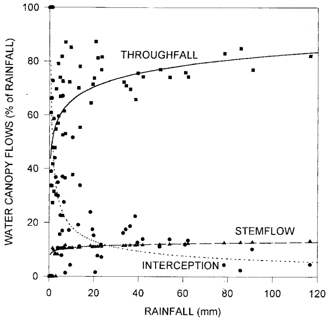
Figure 6. Daily data of the canopy water flows, THF, STF and INT (in percentage of rainfall), and their regression curves with gross precipitation (mm). The fitted equations are the following: THF = 28.84 + 13.82 * \ln(P) , with R^2 = 0.671 and n = 60 ; STF = 3.41 + 2.46 * \ln(P) , with R^2 = 0.763 and n = 60 ; and INT = 57.04 * (P)^{-0.49} , with R^2 = 0.608 and n = 60 .
