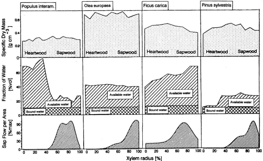
Figure 2. Xylem specific dry mass, water content (volumetric fraction of water) and sap flow rate per area (in percentage of its maximum) in species showing very contrasting radial pattern of all measurement parameters: american poplar ( Populus interamericana cv. Beaupre) as an example of species with higher water content in heartwood then in sapwood, Olea europaea L. with almost equal water content in heartwood and sapwood, Ficus carica L. with gradually increasing water content towards sapwood and Pinus sylvestris L. with larger water content in sapwood then in heartwood.
