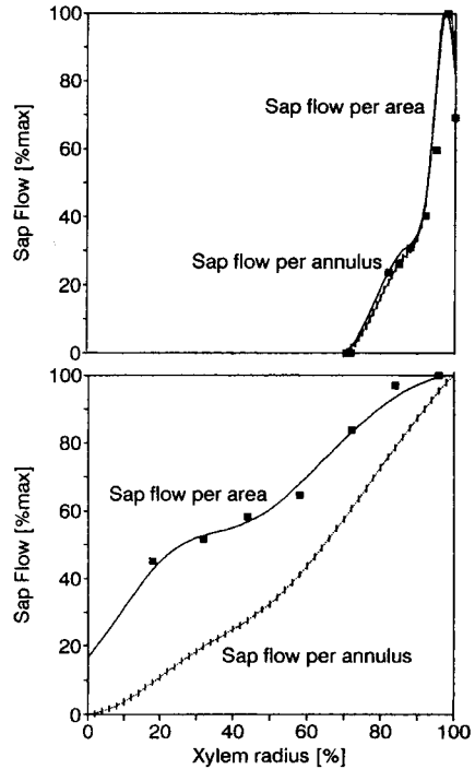
Figure 4. Radial profile of sap flow calculated per unit area and that calculated per entire area of corresponding annuli in trees with relatively shallow (A) and deep sapwood (B).
