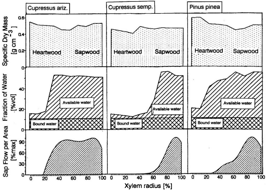
Figure 3. Radial pattern of specific dry mass, xylem water content (volumetric fraction of water) and sap flow rate per area (as a percentage of its maximum) in species with higher water content in sapwood than in heartwood, but different patterns of sap flow. Sap flow occurring virtually over the whole sapwood is demonstrated in the example of Cupressus arizonica Green.; sap flow occupying the prevailing part of the sapwood is shown in Cupressus sempervirens L.D. and sap flow occurring only over part of the sapwood is represented by the example of Pinus pinea L.
