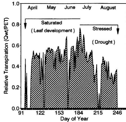
Figure 7. Seasonal course of relative transpiration in large spruce tree ( Picea abies (L.) Karst.) near Rajec, southern Moravia, calculated as the ratio of daily totals of actual transpiration (the sap flow) to potential evapotranspiration, both considered for projected crown area unit. Periods of rather mild and dry weather are marked with horizontal lines. Arrows indicate sampling period of sapwood applied for estimation of the radial xylem water content.
