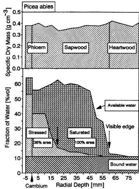
Figure 6. Xylem specific dry mass and tissue water content (volumetric fraction of water) along stem radius at breast height in large spruce tree ( Picea abies (L.) Karst.) with xylem diameter of 31 cm under conditions of saturated tissues in early spring and after a period of severe drought in late summer. The visible edge of sapwood corresponding to higher xylem water content is marked by arrows. Bound water was taken as the percentage of water held in the heartwood (~11 %vol) and available water as that above this value.
