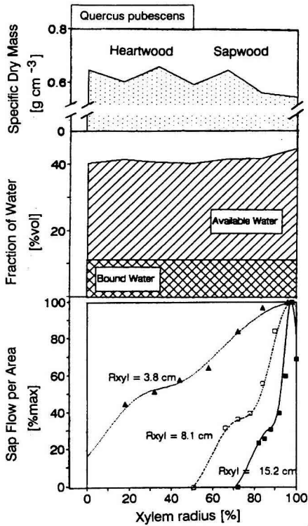
Figure 5. Radial pattern of specific dry mass, xylem water content (volumetric fraction of water) and sap flow rate per area (as a percentage of its maximum) in oak trees ( Quercus pubescens Willd.) of different age (10–40 years) and stem diameter at breast height.
