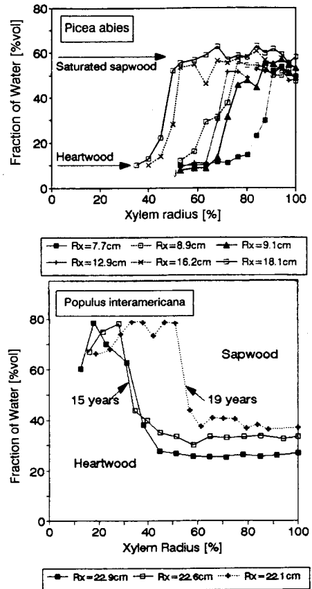
Figure 1. Radial xylem water content (volumetric fraction of water) in species representing contrasting pattern. Six Norway spruce ( Picea abies (L.) Karst.) and three poplar ( Populus interamericana , cv. Beaupre) trees were shown. All spruce trees of large diameter range were about 80 years old, poplar trees were of almost identical diameter, but of different age. Sapwood was saturated in spruce (early spring values), while that of poplar sampled in late summer was not saturated.
