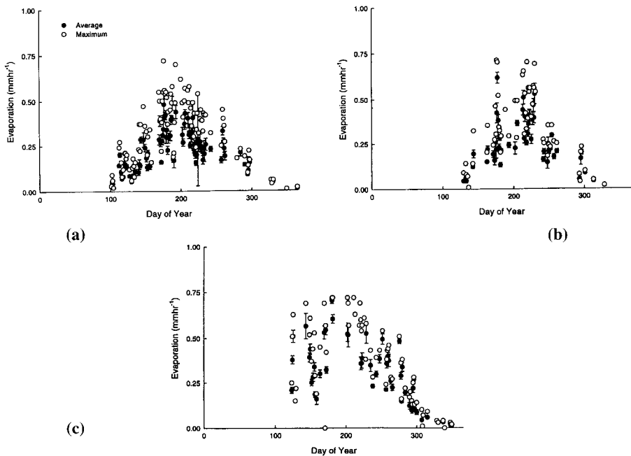
Figure 2. Evaporation rates of the pine forest (a), the larch forest (b) and the poplar forest (c). Maximum rates and average daily rates are given as a function of day of year.
