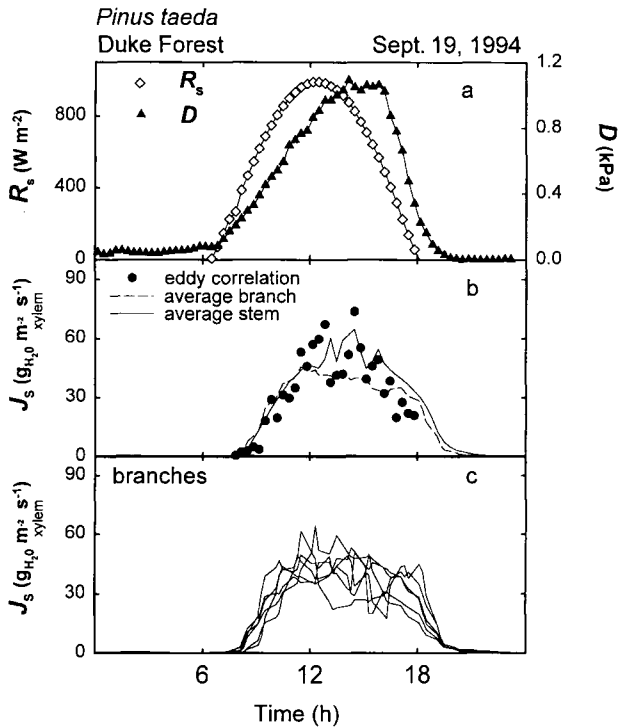
Figure 7. On a clear day, shortwave radiation ( R_S ) showed a nearly symmetrical pattern, while the pattern in vapor pressure deficit, D , lagged relative to the radiation (a). Latent heat flux, LE , obtained with eddy correlation above the canopy, was converted for convenience of comparison with xylem flux, J_S , into similar units (b). The J_S of two trees adjacent to the tower, and their six branches, were compared to LE (b). Individual branches may display large high frequency variability (c), more similar to that measured with eddy correlation.
