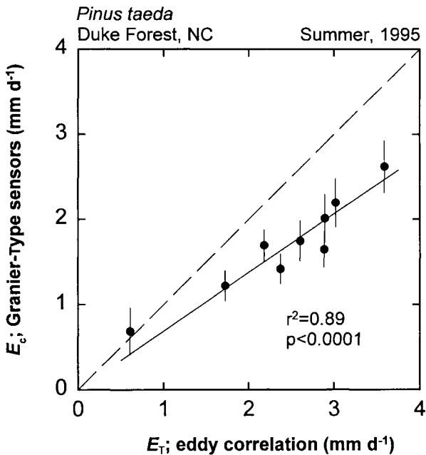
Figure 6. Canopy transpiration, E_C (vertical bars are 1 SE) is compared to total evapotranspiration, E_T , estimated based on eddy correlation measurements. The relationship between the estimates based on the two methods was linear, with a zero intercept ( P > 0.1 ), and was not affected by atmospheric CO 2 concentration. The relationship was E_C = 0.69E_T .
