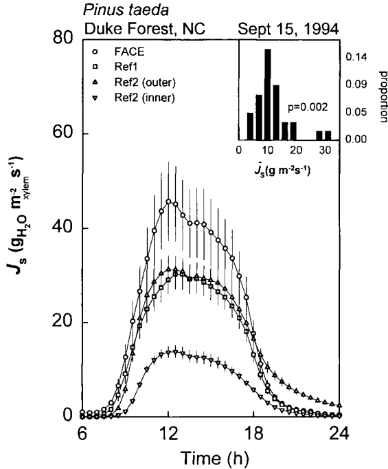
Figure 1. Diurnal pattern of water flux in the xylem ( J_S ) in three clusters of trees in the outer 20 mm of the xylem, and the next 20 mm of the xylem (Ref 2 cluster only). Vertical lines represent 1 SE. Inset: frequency distribution of average diurnal outer J_S combined from the three clusters shows a departure from normality.
