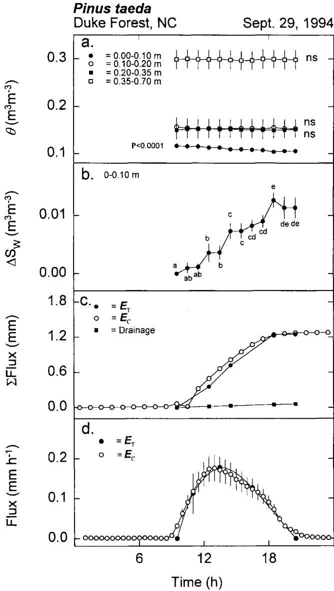
Figure 4. Throughout the day, volumetric soil water content, \theta , in the top soil layer (0–0.1 m; measured with a time domain reflectometer, TDR) changed from 11.65 to 10.52 %, while in the other three layers, to a depth of 0.7 m, \theta remained constant (a). Converting \theta at the top layer to changes in stored water, \Delta S_W , and testing for the difference between the means, identified four distinct means ( P < 0.05 ; b). Cumulative drainage [calculated using equation (3) in text] was very low (0.058 mm; c). A diurnal pattern in canopy transpiration, E_C , was compared as cumulative values (c) or periodic values (d) to total evapotranspiration, E_T , estimated from \Delta S_W and drainage. Vertical bars represent 1 SE, calculated for E_C as described in the text, and for E_T based on the variance between individual TDR rod-pairs.
