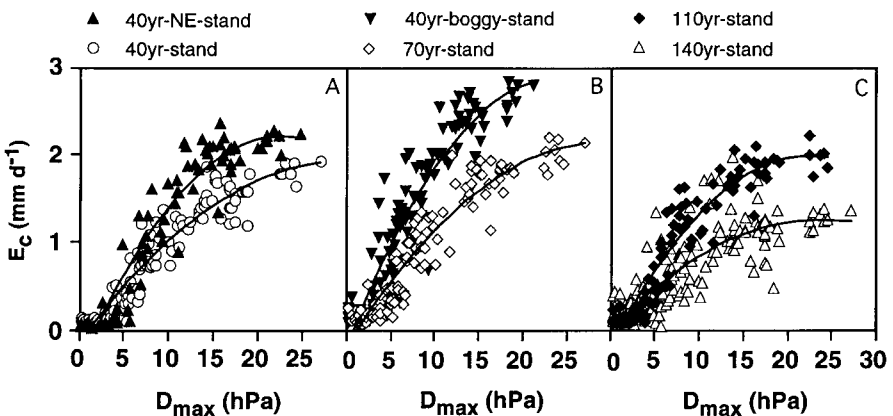
Figure 4. Relation of diurnal integrated tree canopy transpiration ( E_c ) to the daily maximum half-hourly value of vapor pressure deficit ( D_{\max} ) during the measurement period in 1995 at the six investigated spruce stands.
