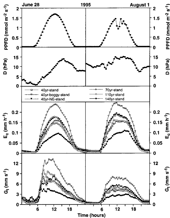
Figure 2. Half-hourly average values of photosynthetic photon flux density (PPFD), vapor pressure deficit ( D ) measured above the canopy at the 140-year stand, tree canopy transpiration of Picea abies ( E_c ) at six experimental sites determined from xylem sapflow, and total tree canopy water vapor transfer conductance ( G_t ) on 28 June and 1 August 1995. The time courses for sap flow rate were adjusted by 0.5–1.5 h (to achieve compatibility between morning increases in PPFD and E_c ) to compensate for the capacitive delay in flow detection at breast height as compared to crown level transpiration. G_t was estimated from shifted E_c and D as described by Köstner et al. [32].
