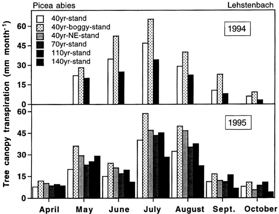
Figure 6. Seasonal variation during summer 1994 and 1995 in the monthly sum of tree canopy transpiration measured by xylem sapflow measurements at the experimental spruce sites at the Lehstenbach catchment. In 1994 measurements only took place at three of the six experimental sites and an estimation of transpiration rates in April was not possible.
