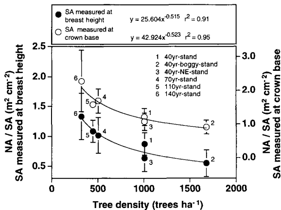
Figure 10. Relationship between tree density and the mean ratio of needle area (NA) to sapwood area (SA) of the harvested trees from each of the investigated spruce stands (error bars: standard error). Relationship is shown for SA measured at breast height and at crown base.
