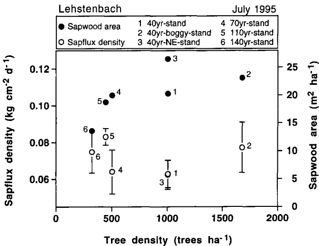
Figure 8. Mean sapflux density (transpiration per sapwood area; open circles) of 10–12 individual trees in each stand and cumulative sapwood area at breast height (solid circles) related to stand tree density (error bars: standard error). The values shown for sapflux density are averages for July 1995.
