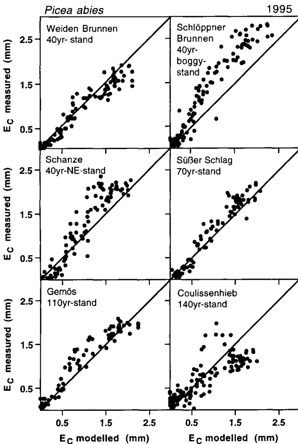
Figure 11. Comparison of measured and simulated daily integrated tree canopy transpiration rates for the six experimental spruce stands studied in 1995 in the Lehstenbach catchment. The assumptions of the model (STANDFLUX, [15]) include a single needle physiology, a single average tree structure defined for each stand, and variation among stands due to tree density (overall r^2 = 0.82 ).
