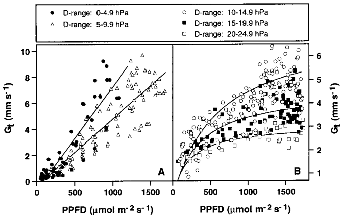
Figure 3. Analysis of the influence of photon flux density (PPFD) and vapor pressure deficit ( D ) on total tree canopy water vapor conductance ( G_t ) with the aid of non-linear regression techniques at the 40-year stand. At low D (up to 10 hPa) G_t was linearly correlated to incident PPFD (A), while at higher D G_t saturates with increasing PPFD (B). The solid lines indicate the linear regressions and the results of the non-linear model (equation of form: G_t = 1/(a*(1/PPFD) + b*D) ).
