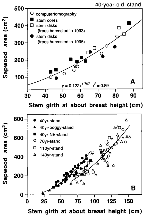
Figure 9. A: Correlation between stem girth at ca breast height and cross-sectional sapwood area at the same height determined either by measurements of sapwood from stem disks of harvested trees or with stem cores or by computer tomography at the 40-year stand (data of the trees harvested in 1995 were obtained by M. Mund; unpublished). B: Correlation between stem girth at ca breast height and cross-sectional sapwood area at the same height determined at the three 40-year-old stand and in the older stands.
