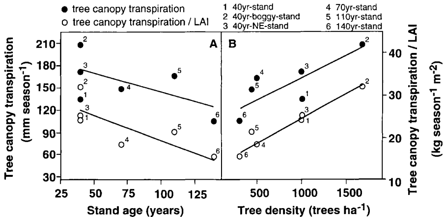
Figure 7. Correlation between stand age and tree density of the six investigated stands and seasonal total of tree canopy transpiration (absolute values as well as standardized on the basis of projected stand leaf area index).
