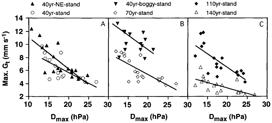
Figure 5. Relation of maximum total tree canopy water vapor transfer conductance ( G_t ) to the daily maximum half-hourly value of vapor pressure deficit ( D_{max} ) on sunny days during the period from the end of June to end of August in 1995 at the six investigated spruce stands.
