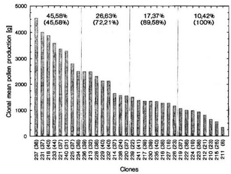
Fig 3. The contribution of individual clones in total pollen production of the orchard averaged over 3 years of observations. Numbers of ramets of respective clones are given in parentheses.
