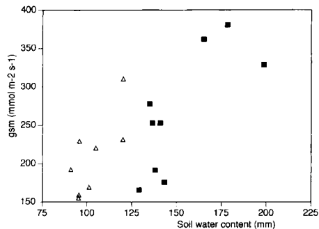
Fig 8. Relationship between soil water content (upper 110 cm) and maximum daily stomatal conductance ( g_{sm} ). \Delta : dry site; \blacksquare : wet site.
