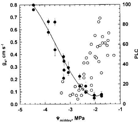
Fig 4. Percent loss hydraulic conductivity (PLC) due to xylem embolism (closed circles) and mid-day stomatal conductance ( g_s ) (open circles) versus leaf water potential at midday ( \Psi_{\text{midday}} ). Vertical error bars represent one standard deviation. Embolism significantly increased in petioles and twigs when \Psi_{\text{leaf}} became lower than -2.7 MPa, the point where the g_s was reduced to about 10% of its maximal value.
