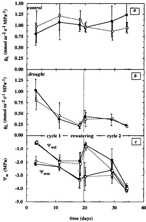
Fig 3. Water relations of inoculated (●) and non-inoculated (○) saplings of Q. robur during 2 successive drought cycles: time-course of leaf specific hydraulic conductance ( g_L ) of well-watered (a) and drought-exposed (b) saplings, and of mid-day ( \psi_{wm} ) and predawn ( \psi_{wd} ) leaf water potentials of drought-exposed saplings (c). Vertical bars indicate standard error.
