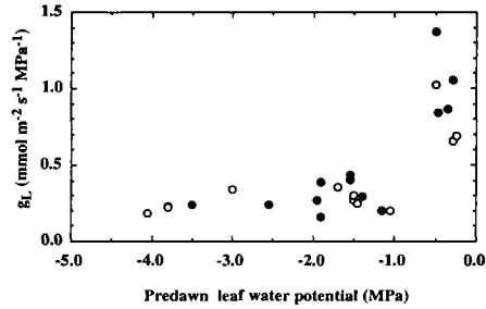
Fig 4. Total leaf specific conductance ( g_L ) of drought-exposed saplings of Q. robur as a function of predawn leaf water potential ( \psi_{wd} ). The data are the same as in figure 2b, but each point represents an individual measurement. Data obtained the day following rewatering were omitted.
