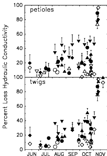
Fig 6. Seasonal progression of xylem embolism in petioles (upper section) and 1-year old twigs (lower section) for both control (open symbols) and water stressed trees (filled symbols). Different trees are represented by the same symbols as in figure 5.
