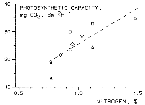
Fig. 2. Photosynthetic capacity as a function of nitrogen content. Symbols refer to different sites. y = 25.3x + 0.1 , R^2 = 0.62 .
