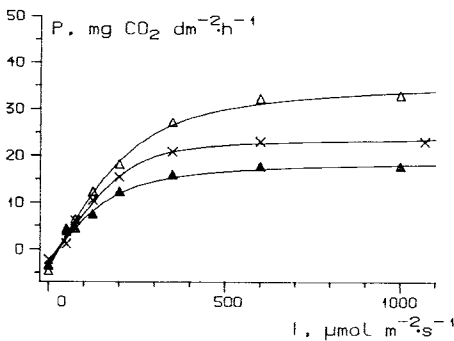
Fig. 1. Photosynthetic radiation response of 3 shoots of different nitrogen status: 1.48% ( \Delta ), 0.93% ( \times ) and 0.77% ( \blacktriangle ).
