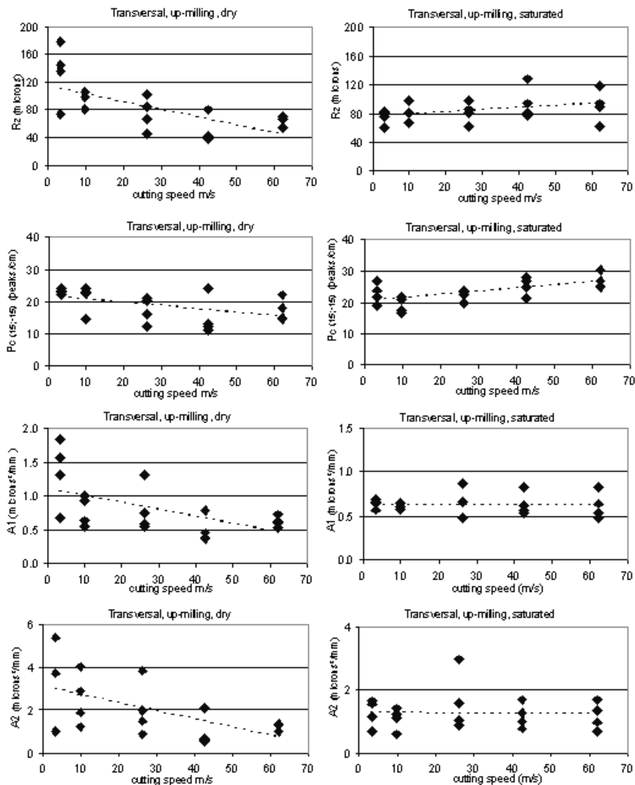
Figure 8. Roughness results for transversal cutting direction and up-milling process.
