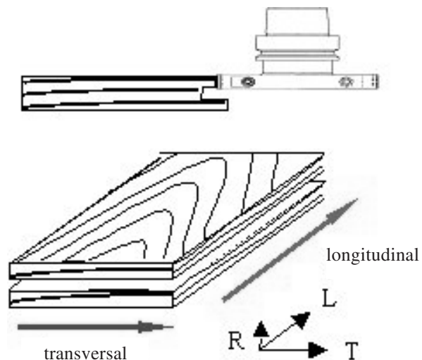
Figure 4. Wood piece shape and cutting directions. Annual rings are orthogonal to the longitudinal side of the piece.
