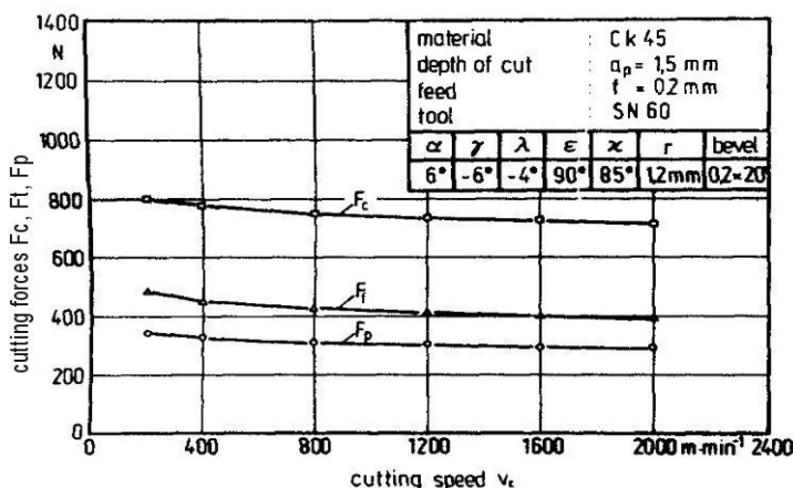
Figure 1. Cutting forces function of cutting speed [28].
