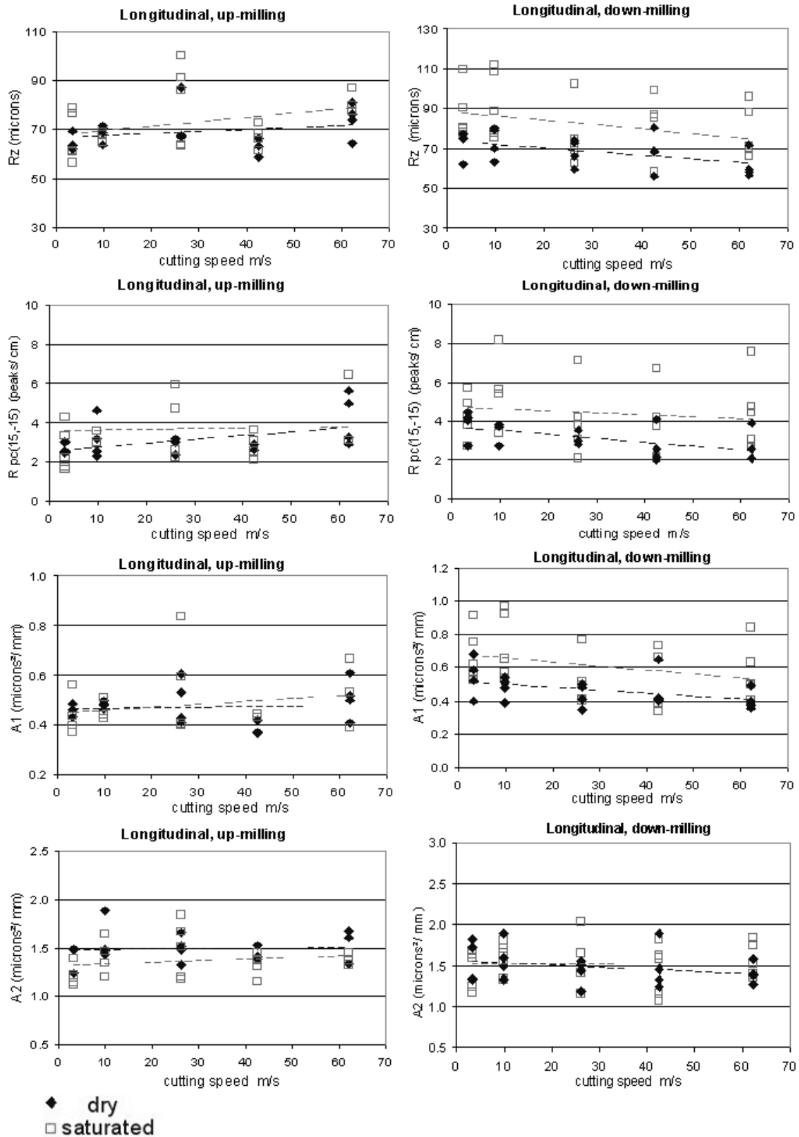
Figure 7. Roughness results for longitudinal cutting.
