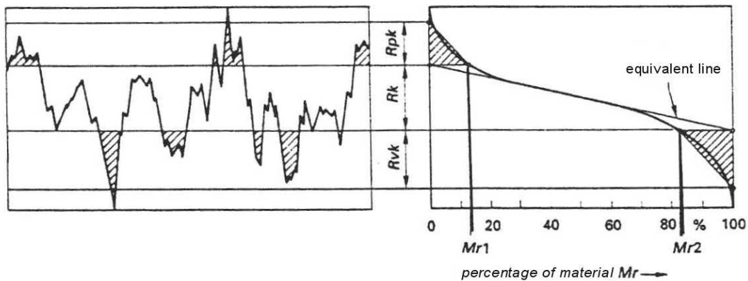
Figure 6. Abbot curve and peaks/valleys areas components. The plotted curve on the right is the height of a virtual cut versus the percentage of material.
