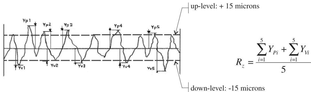
Figure 5. Surface profile with mean line and up- and down-level lines. R_z is the average of the five highest peaks and the five lowest valleys.
