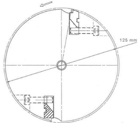
Figure 3. Single tooth tool-holder. The removed tooth has been replaced by an equal weight steel piece (hatched area)
